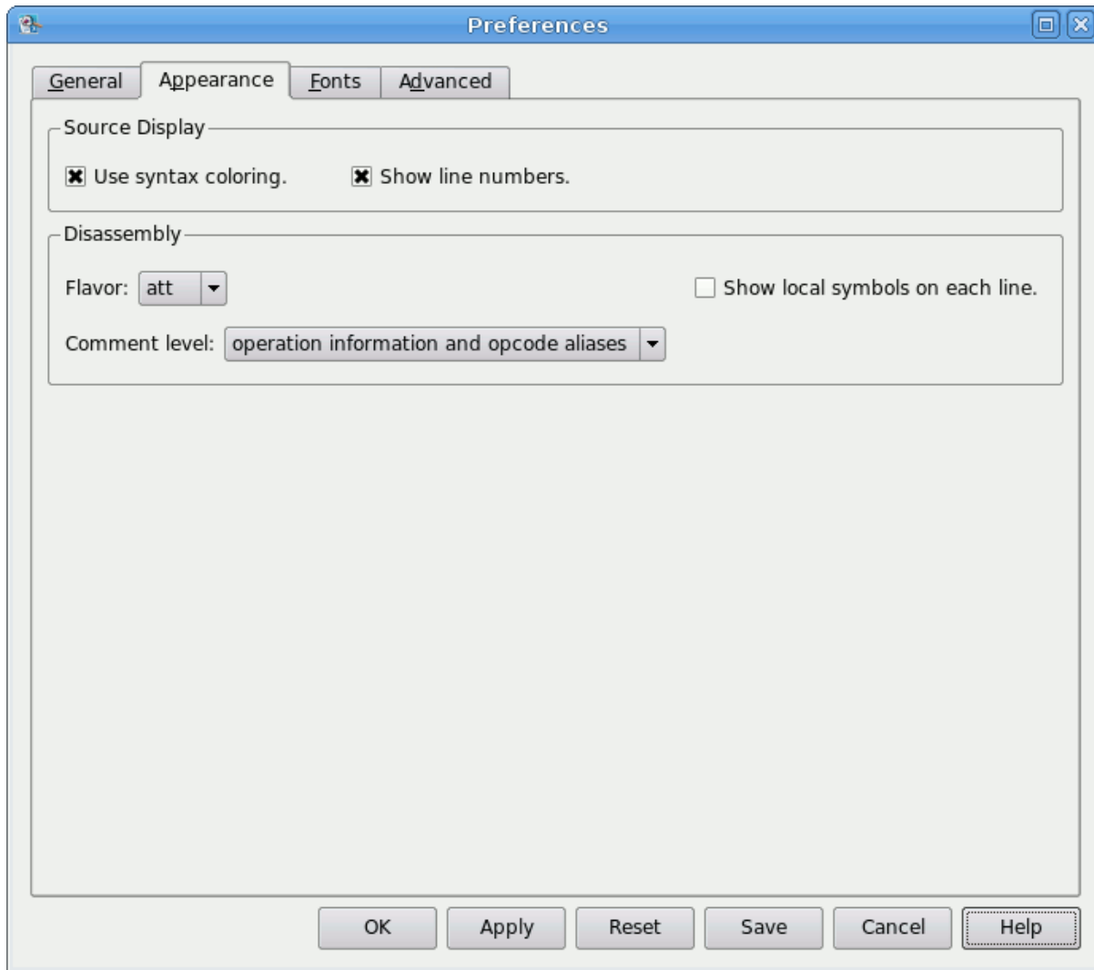
Figure 9-1. Preferences Appearance Page
