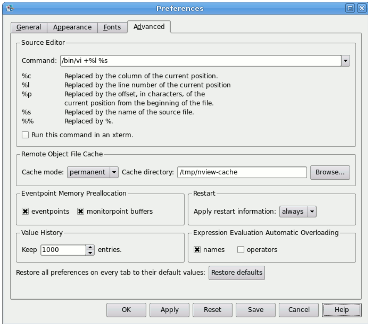
Figure 9-4. Preferences Advanced Page
