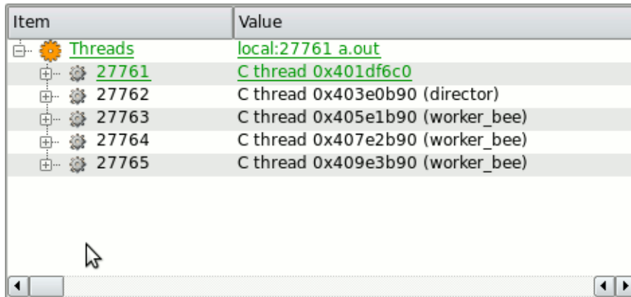
Figure 4-18. Trace Tutorial - director and worker_bee threads
