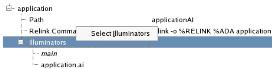
Figure 4-40. Illuminators Context Menu
