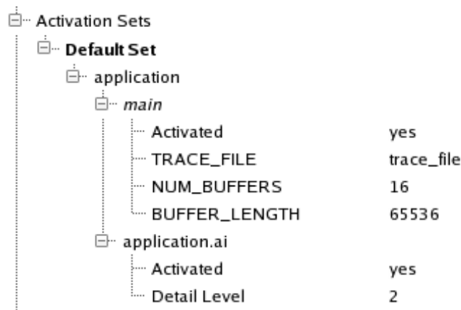
Figure 4-44. Default Options on Illuminators
