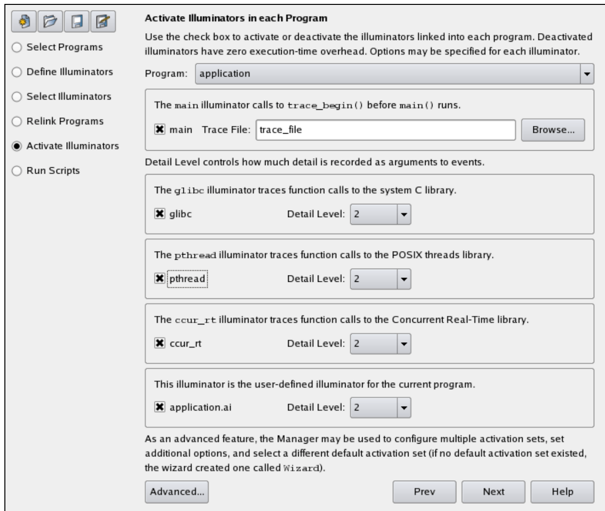
Figure 4-18. Activate Illuminators in each Program Dialog
