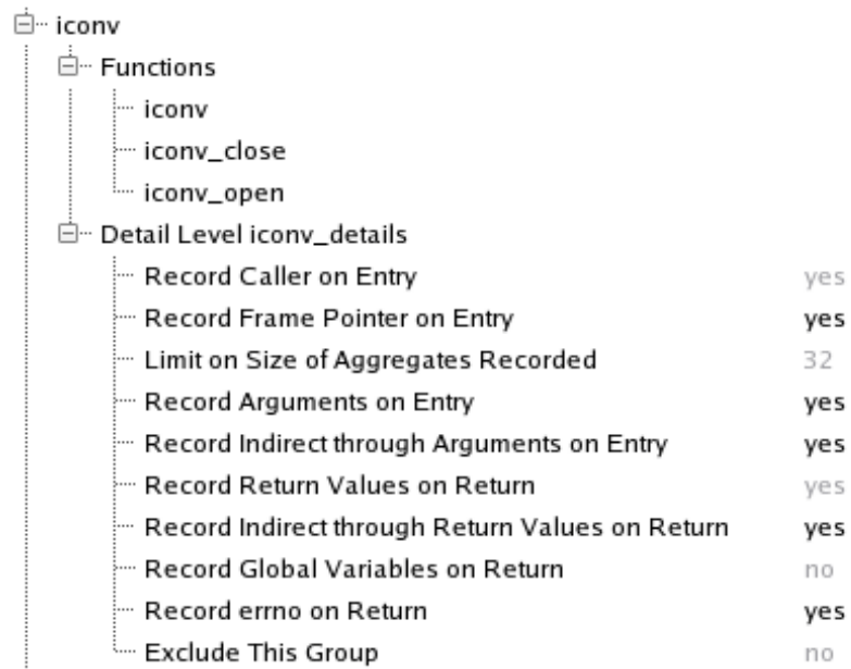
Figure 4-77. A Customized Custom Detail Level for a Group
