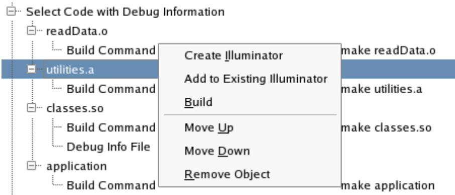
Figure 4-29. Context Menu on an Object
