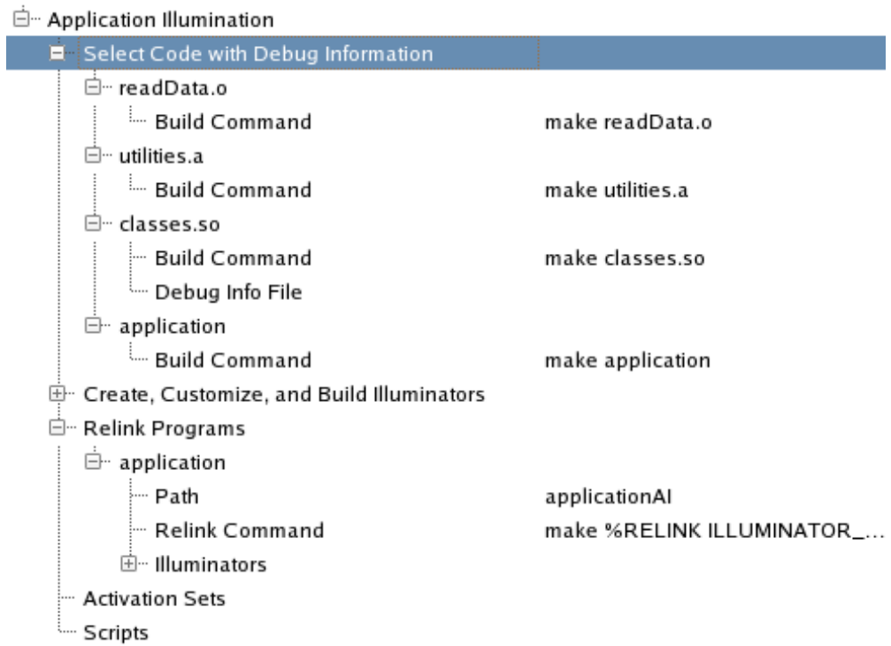
Figure 4-28. Various Objects Added to the Session Manager
