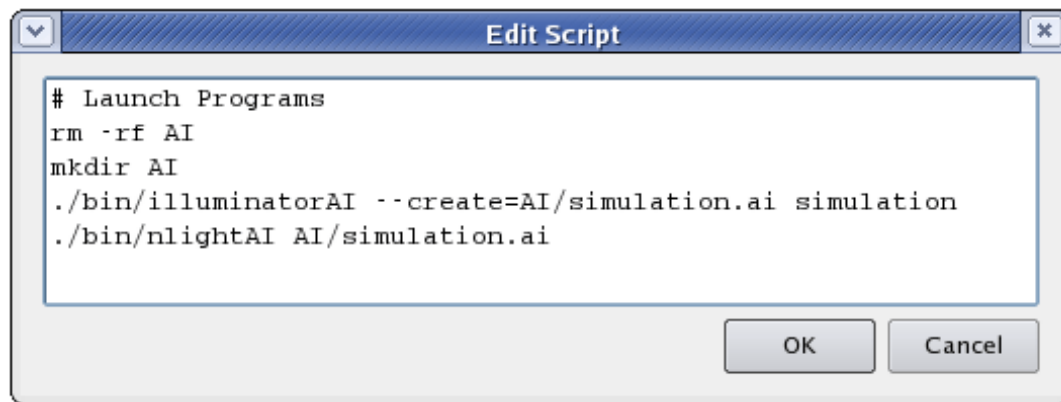
Figure 4-59. Modified Script Launching Instrumented Programs
