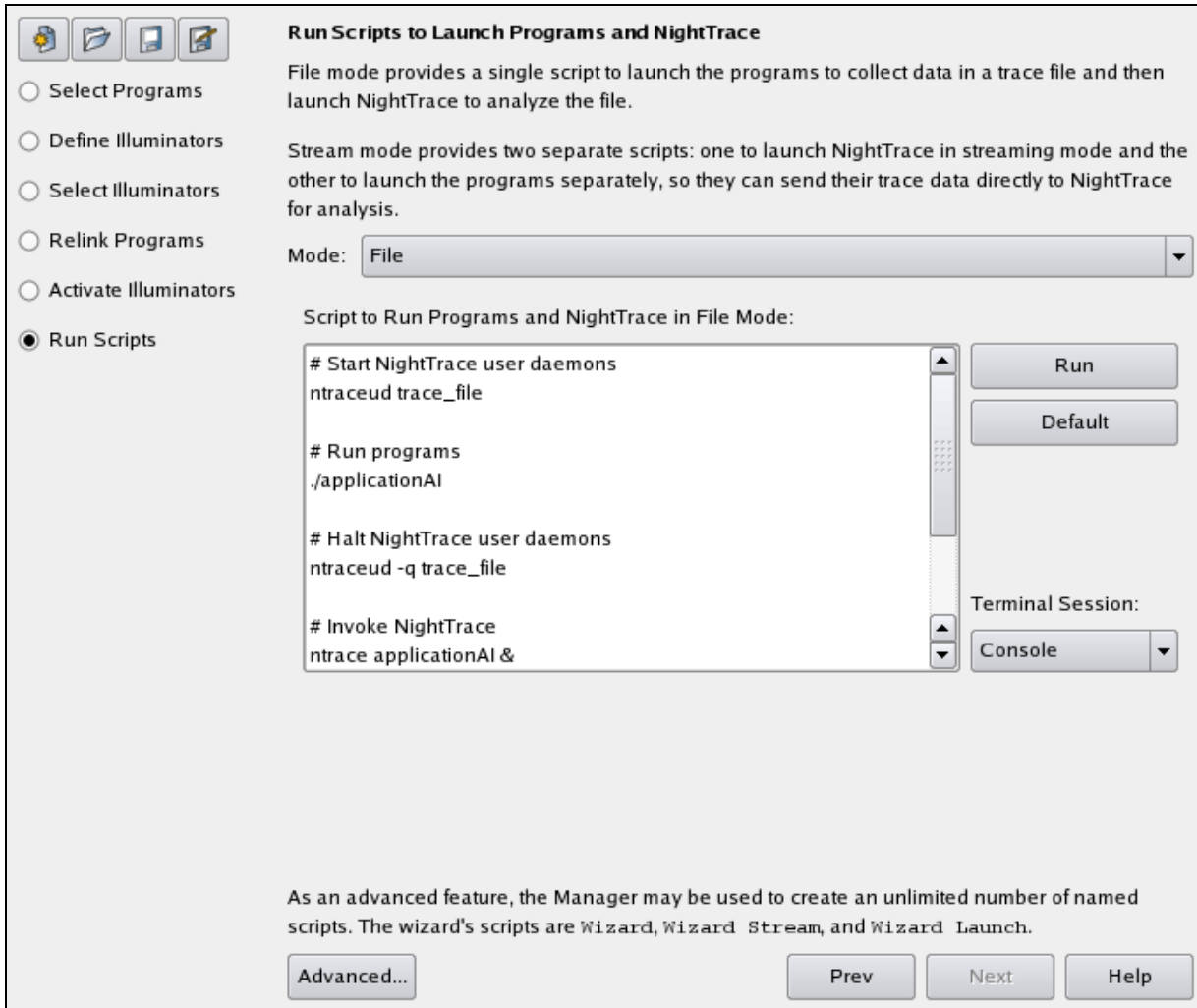
Figure 4-21. Run Scripts to Launch Programs and NightTrace Dialog in File Mode
