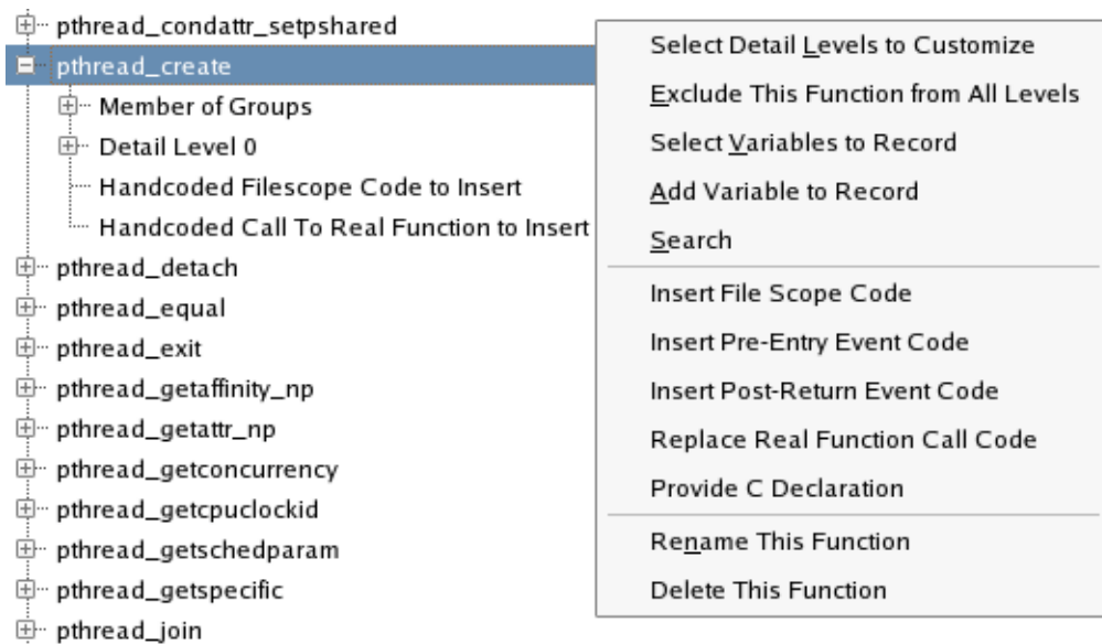
Figure 4-82. Function Context Menu
