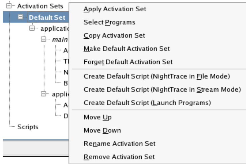
Figure 4-49. Context Menu on an Activation Set
