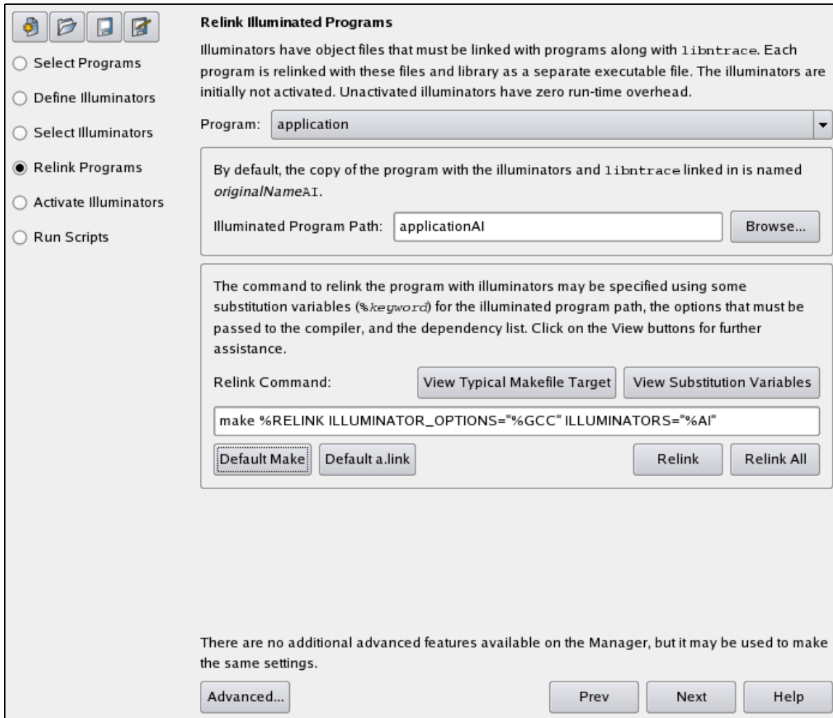
Figure 4-16. Relink Illuminated Programs Dialog
