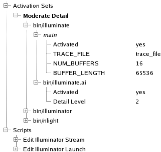
Figure 4-56. Activation Set for an Elaborate Script Example
