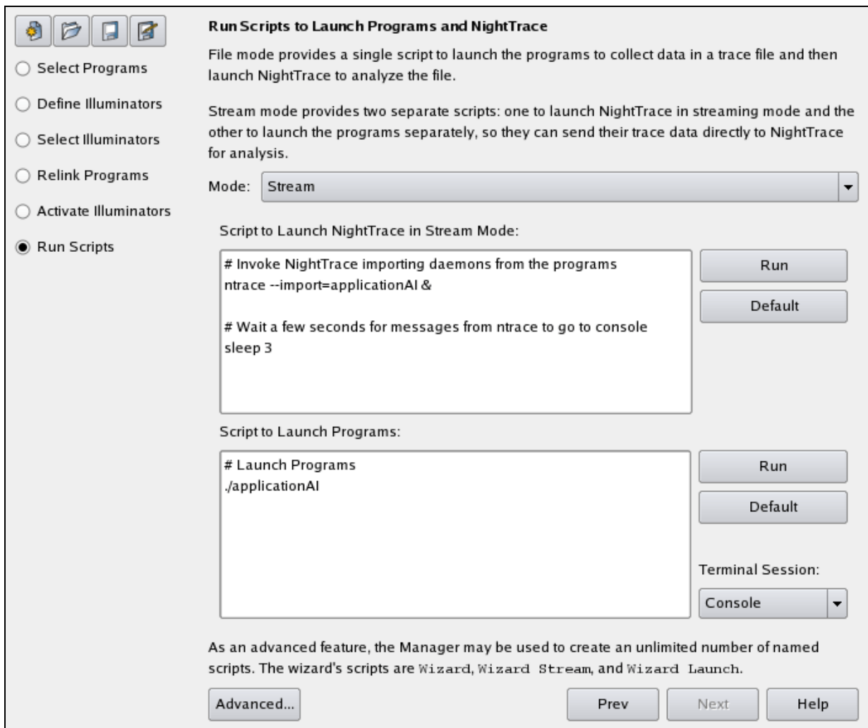
Figure 4-22. Run Scripts to Launch Programs and NightTrace Dialog in Stream Mode
