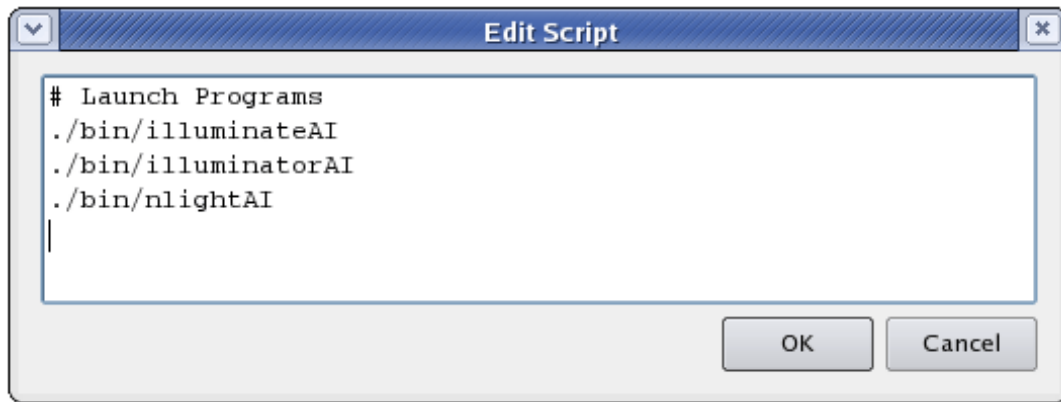
Figure 4-58. Script Launching Instrumented Programs
