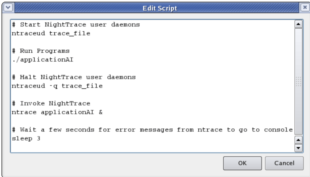
Figure 4-55. Default Script created for an Activation Set (NightTrace in File Mode)
