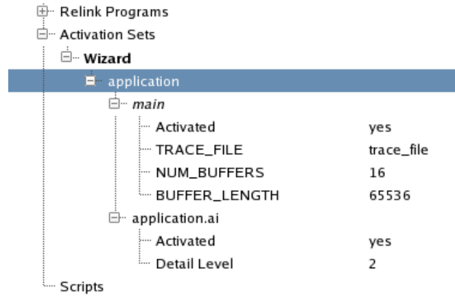
Figure 4-20. Activation Sets Advanced Settings
