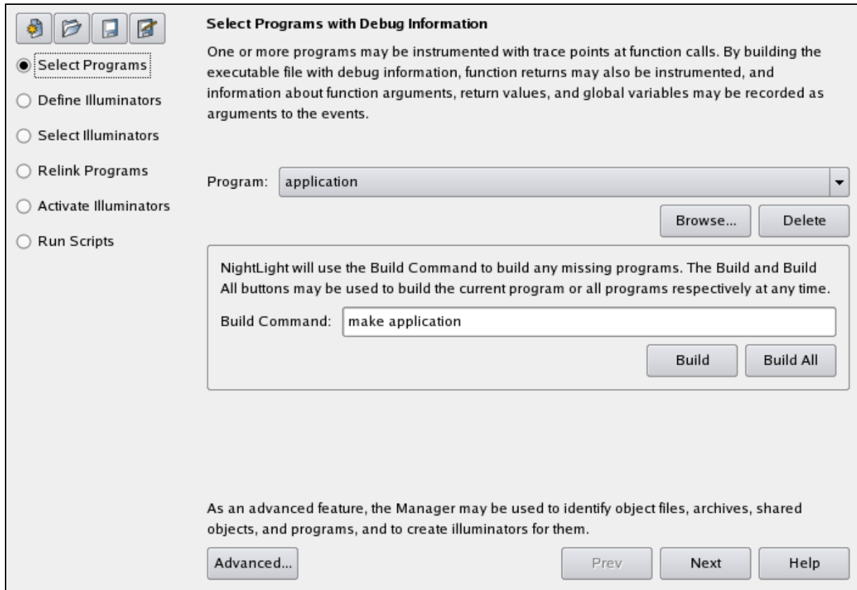
Figure 4-9. Select Programs with Debug Information Dialog
