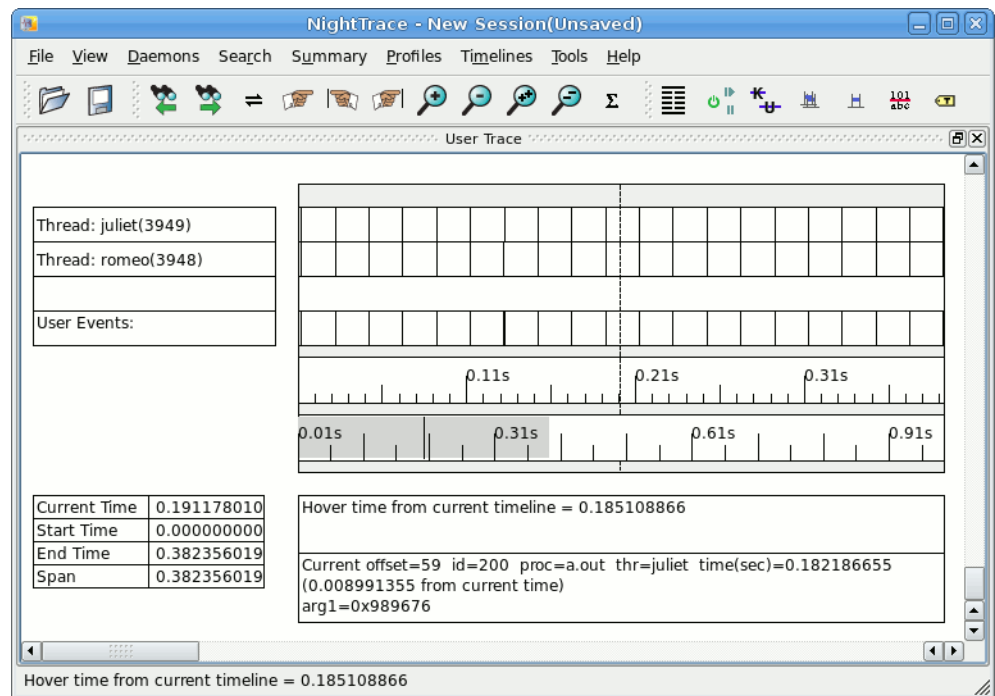
Figure C-1. Automatically Generated Data Display Page
