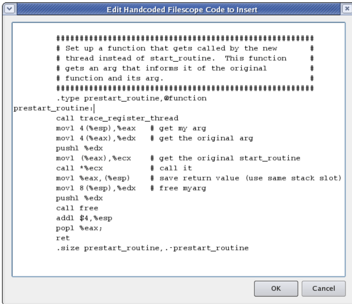
Figure 4-84. Edit Handcoded Dialog
