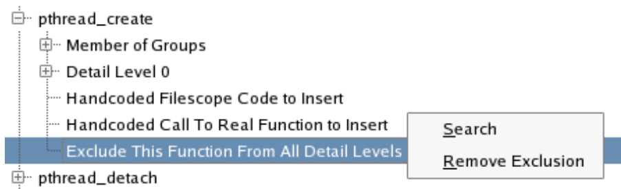
Figure 4-83. Remove Exclusion Context Menu Item
