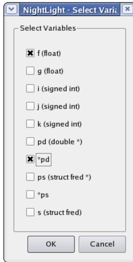
Figure 4-72. Select Variables to Record Dialog
