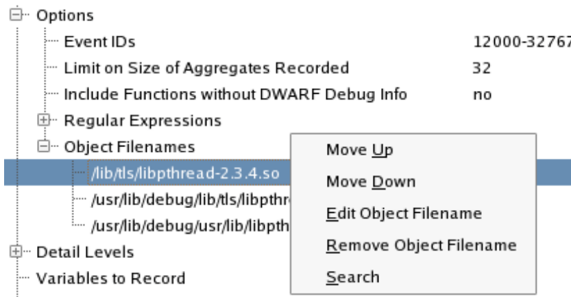
Figure 4-68. Object Filename Context Menu
