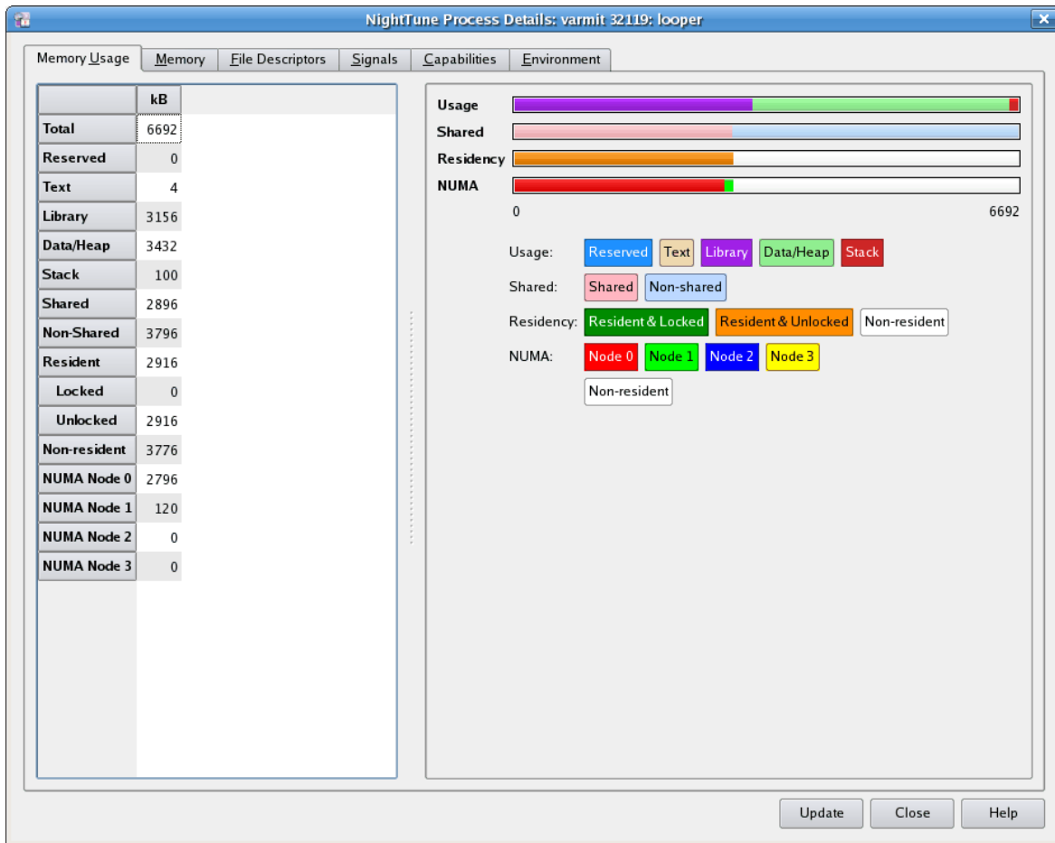
Figure 3-47. Process Details Memory Usage Tab
