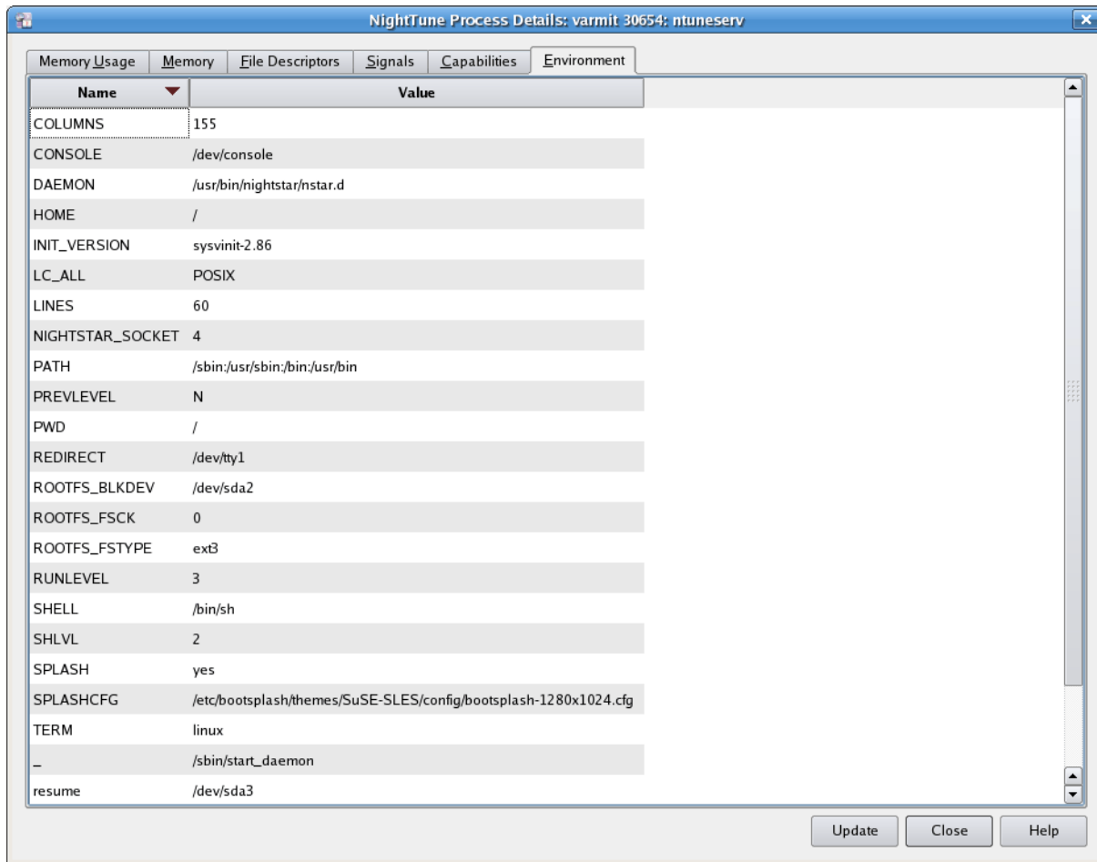
Figure 3-52. Process Details Environment Tab
