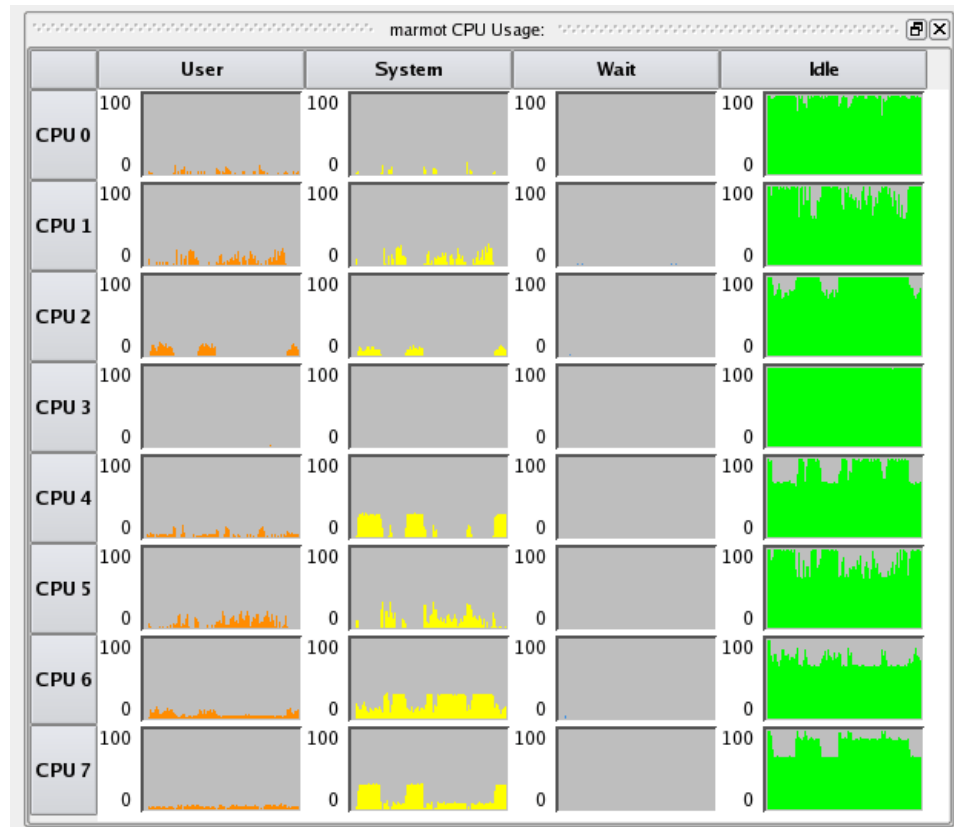
Figure 3-9. CPU Usage Line Graph Pane
