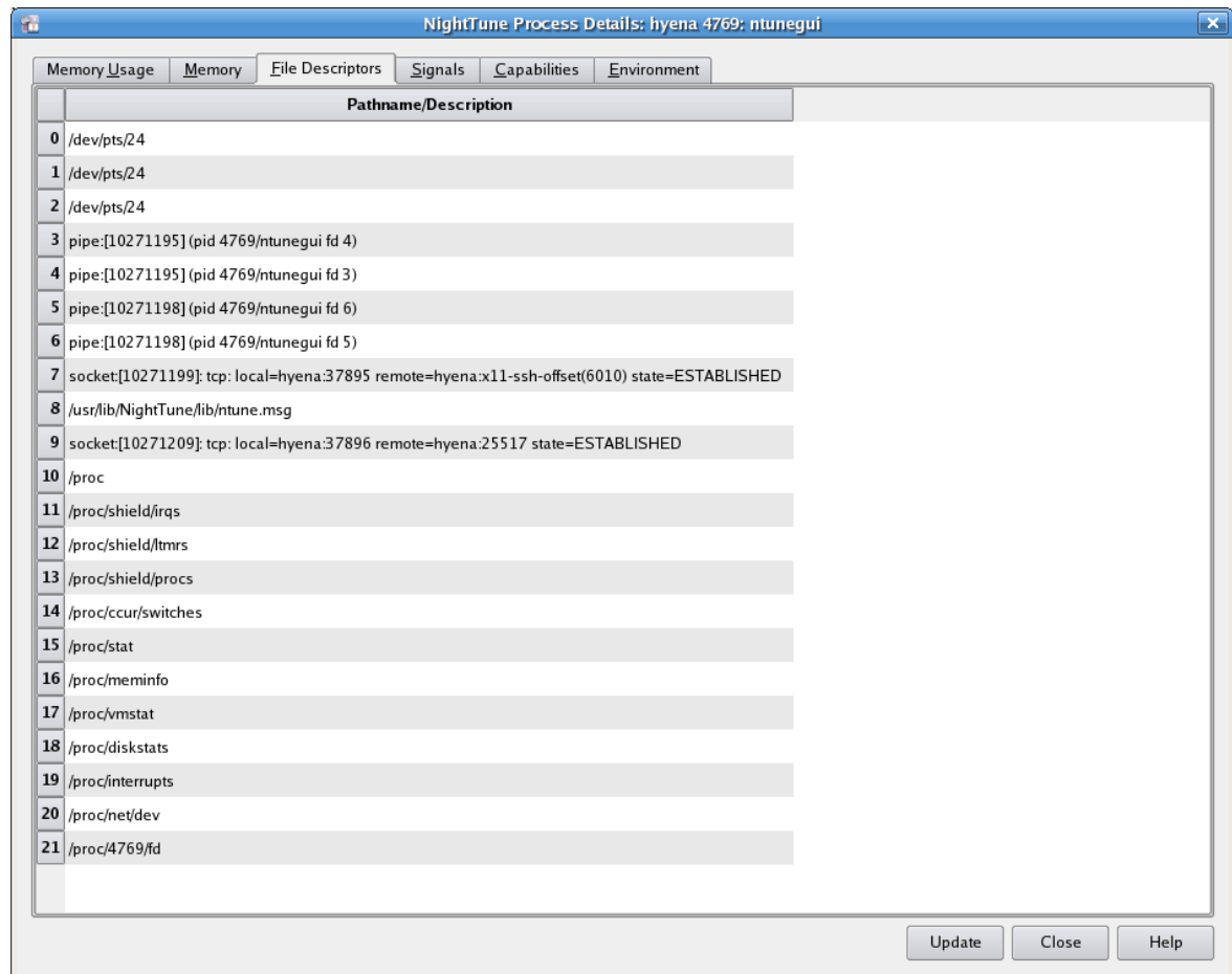
Figure 3-49. Process Details File Descriptors Tab
