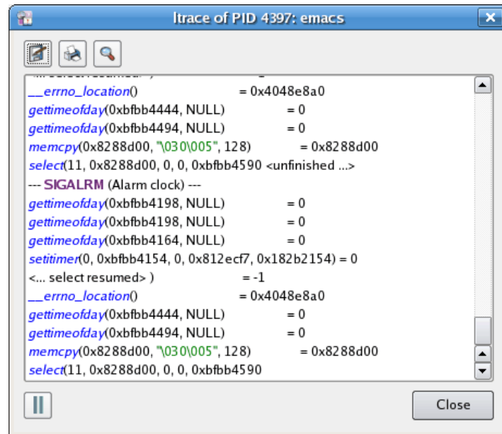
Figure 3-45. Trace Library Calls Window
