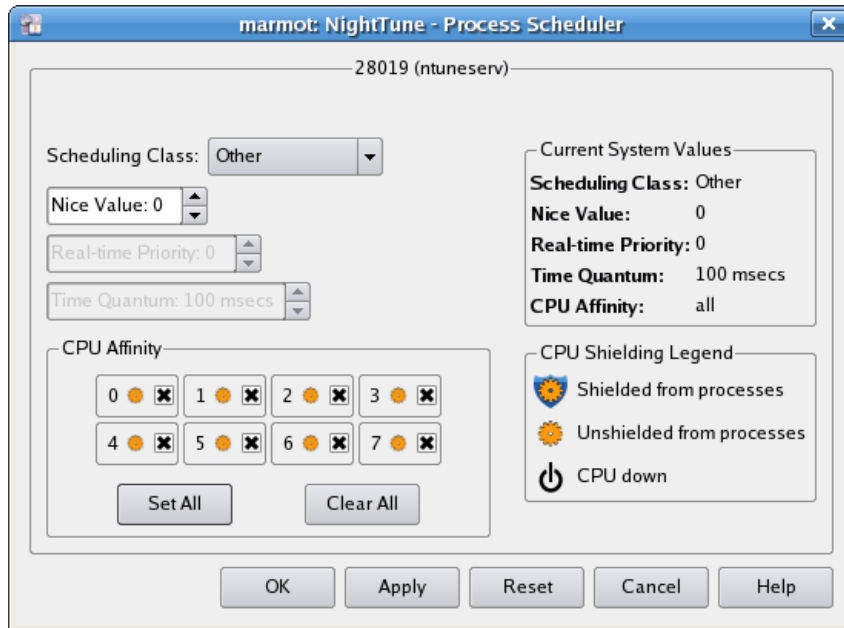
Figure 3-46. Process Scheduler Dialog
