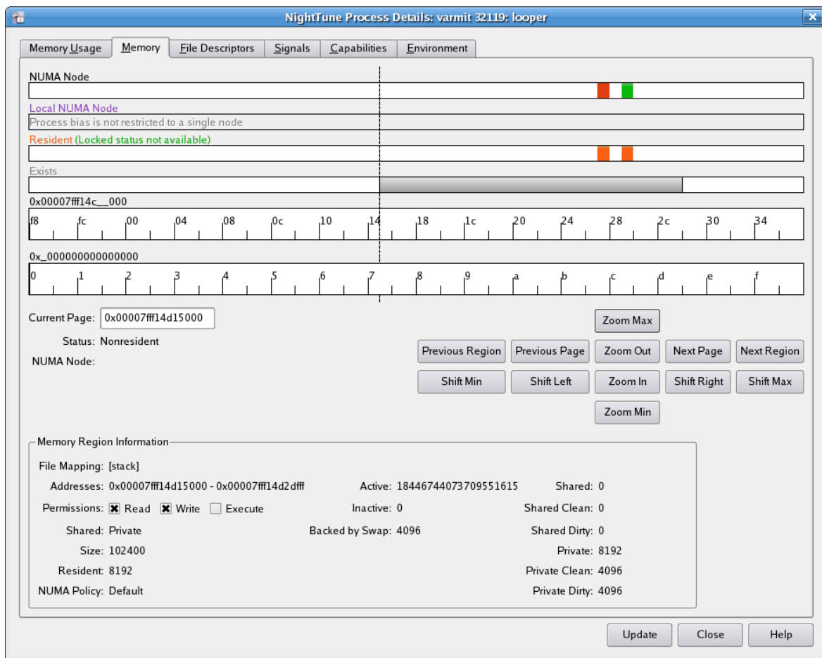
Figure 3-48. Process Details Memory Tab
