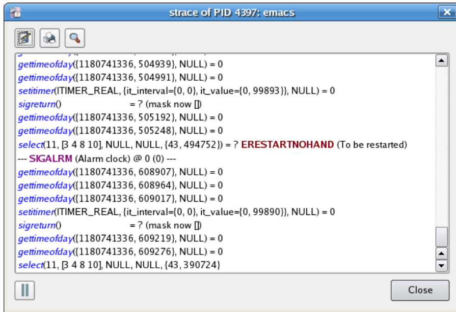
Figure 3-44. Process List Trace System Calls Window
