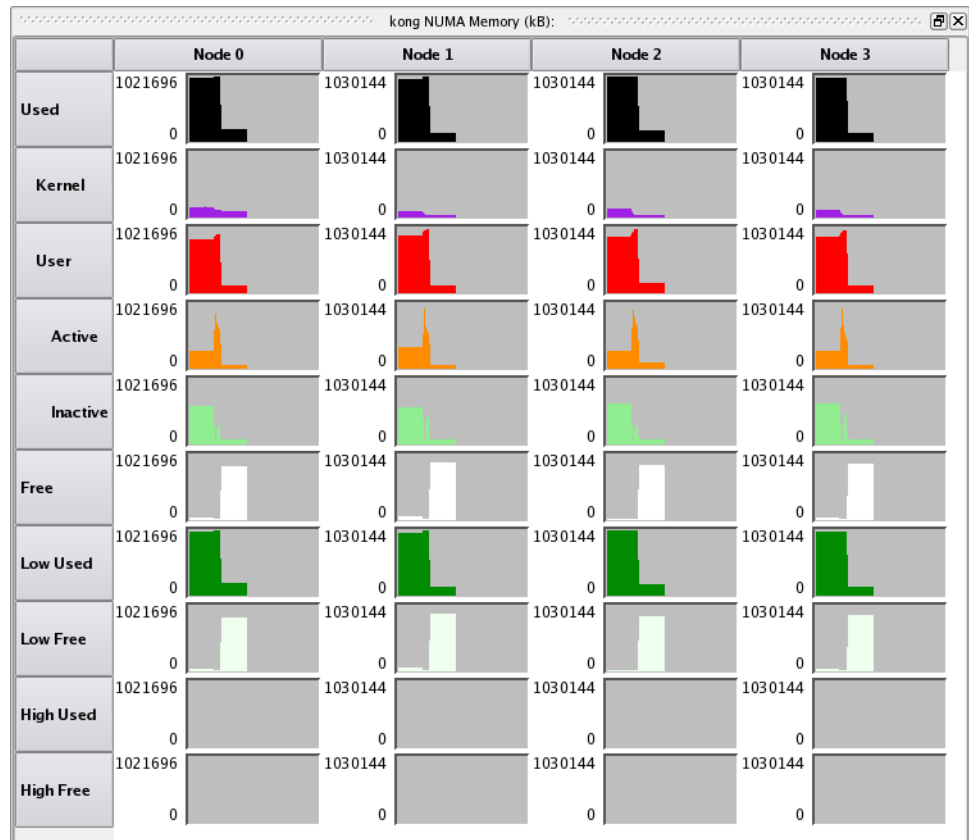
Figure 3-35. NUMA Line Graph Pane
