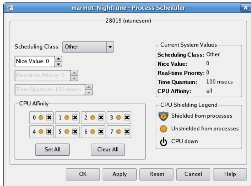
Figure 4-5. Process Scheduler Dialog
