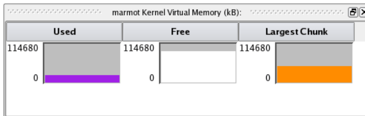
Figure 3-27. Kernel Virtual Memory Line Graph Pane
