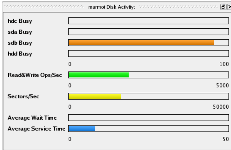
Figure 3-13. Disk Activity Bar Graph Pane
