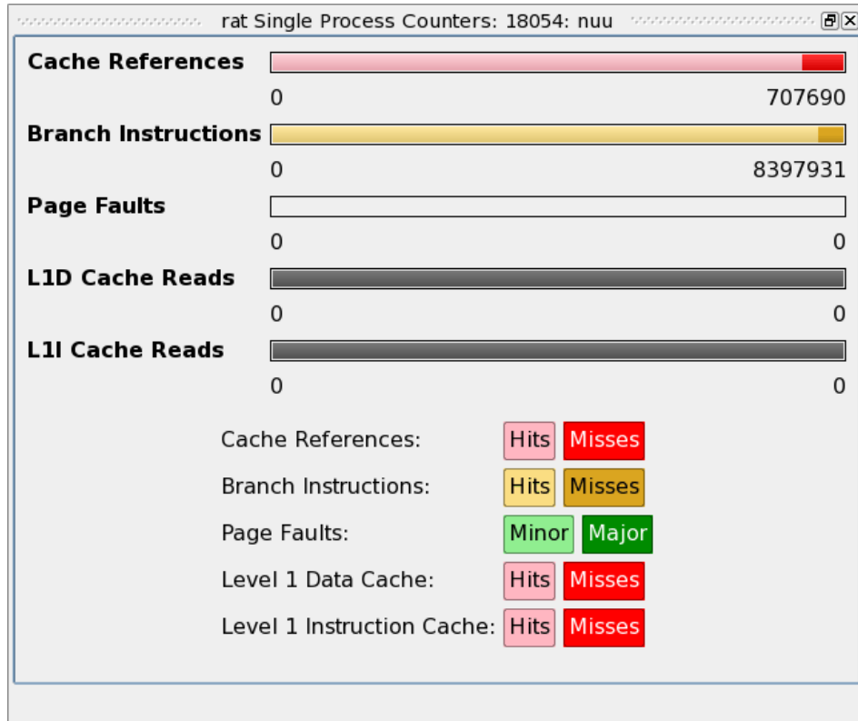
Figure 3-65. Single Process Counters Bar Graph Pane
