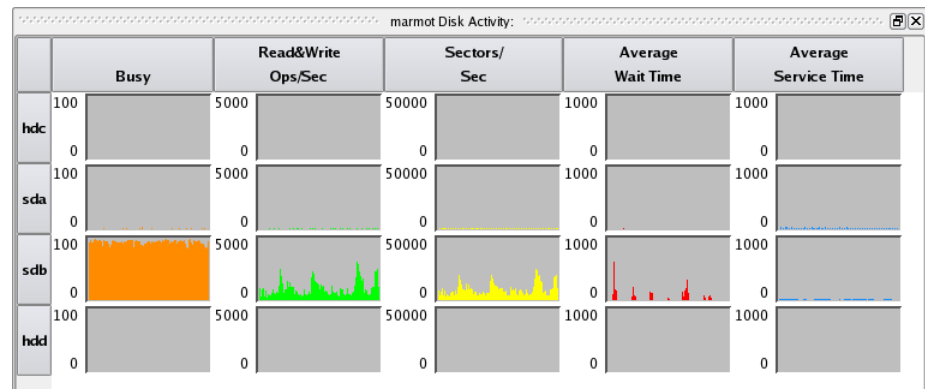
Figure 3-14. Disk Activity Line Graph Pane
