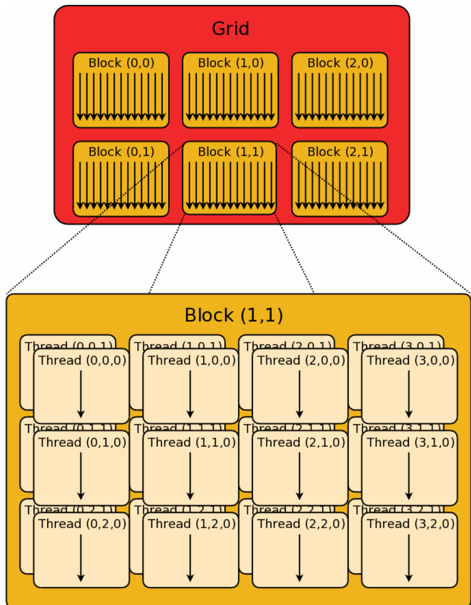
Figure 3-11. Grid, Block, and Thread Hierarchy for \langle\langle (3, 2), (4, 3, 2) \rangle\rangle
