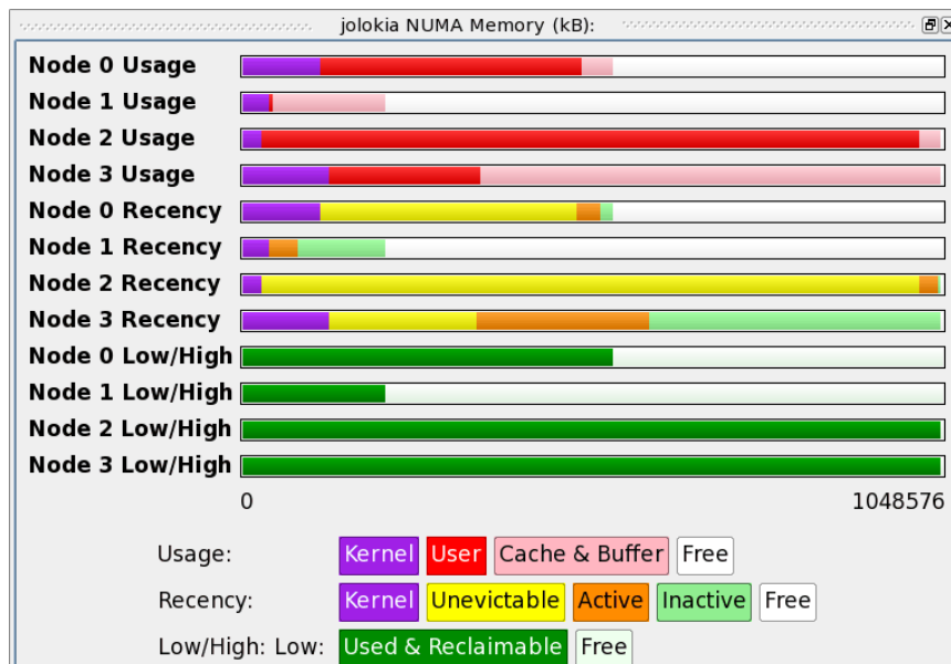
Figure 3-38. NUMA Bar Graph Pane
