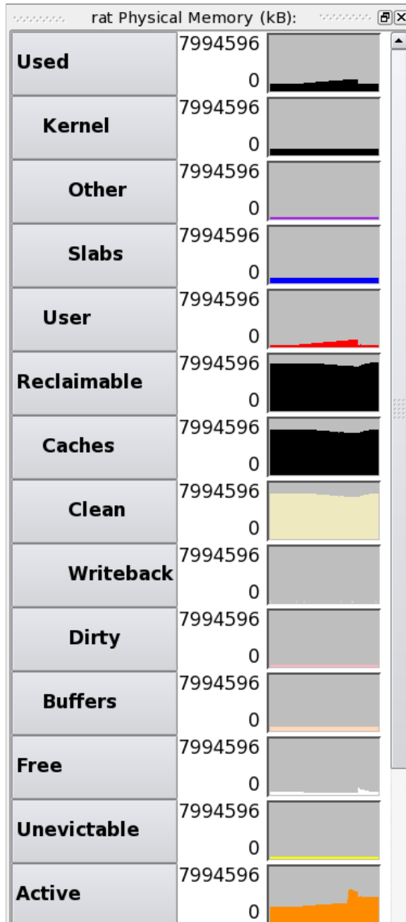
Figure 3-30. Physical Memory Line Graph Pane
