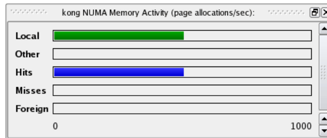
Figure 3-41. NUMA Activity Bar Graph Pane
