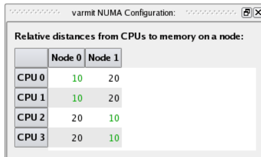
Figure 3-44. NUMA Configuration Distance Pane
