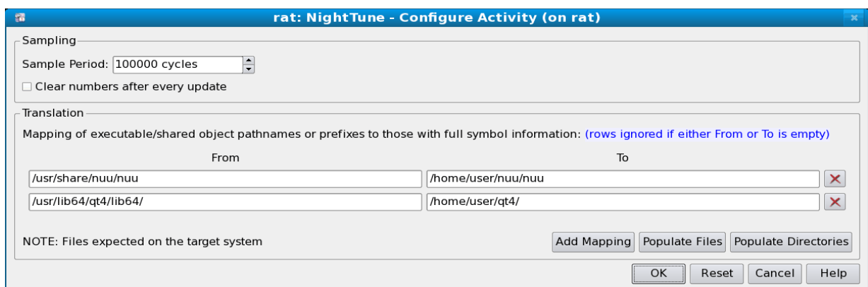
Figure 3-63. Single Process Configure Activity Dialog
