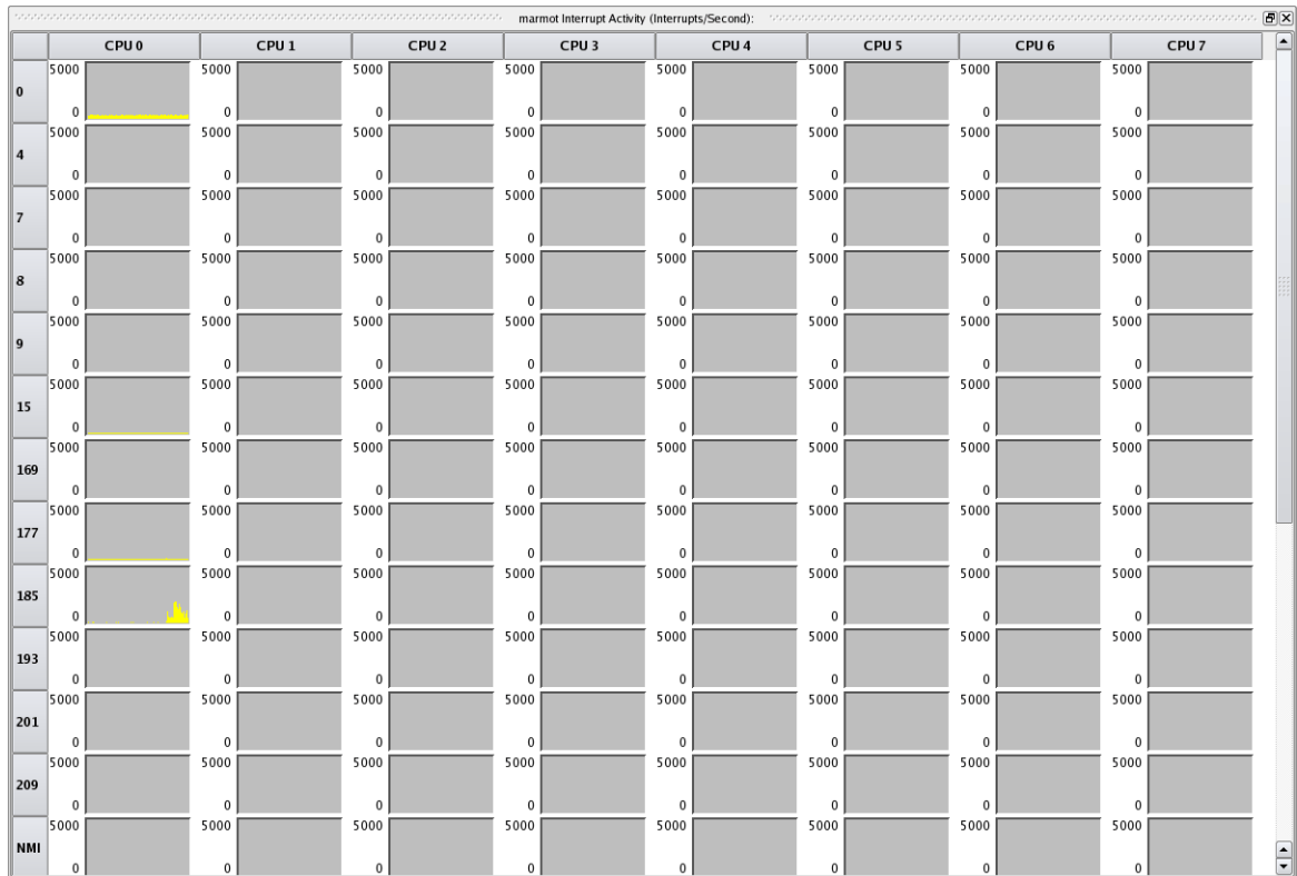
Figure 3-17. Interrupt Activity Line Graph Pane
