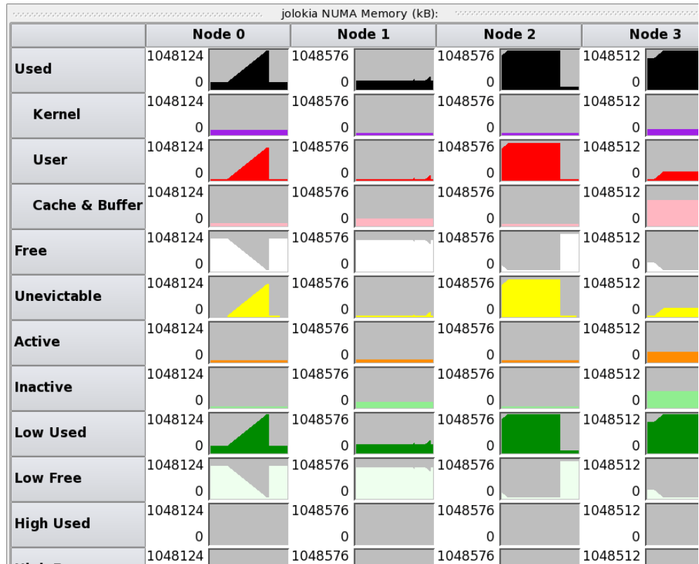
Figure 3-39. NUMA Line Graph Pane
