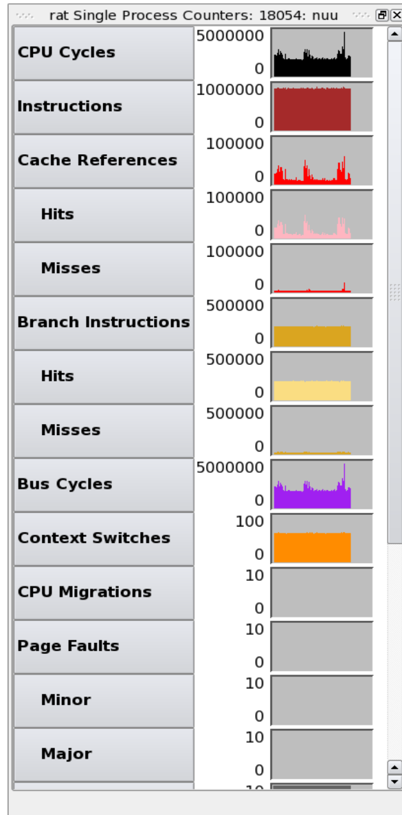
Figure 3-66. Single Process Counters Line Graph Pane
