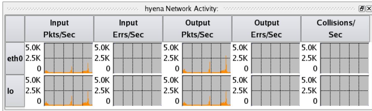
Figure 3-41. Network Activity Line Graph Pane
