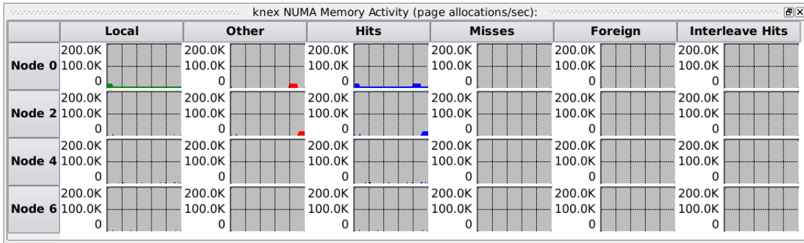
Figure 3-47. NUMA Activity Line Graph Pane
