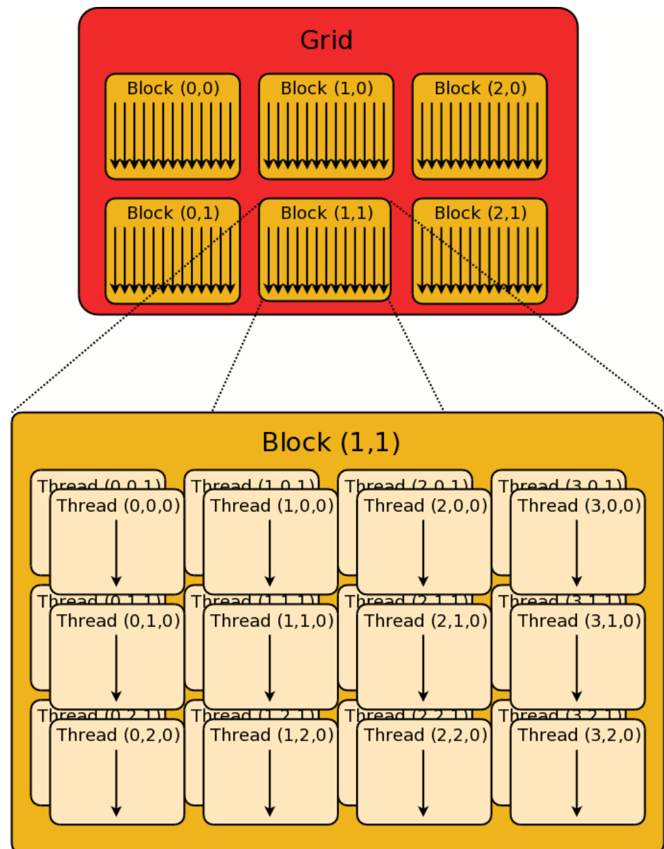
Figure 3-16. Grid, Block, and Thread Hierarchy for \langle\langle 3, 2 \rangle, \langle 4, 3, 2 \rangle \rangle
