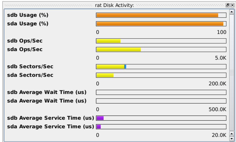
Figure 3-18. Disk Activity Bar Graph Pane
