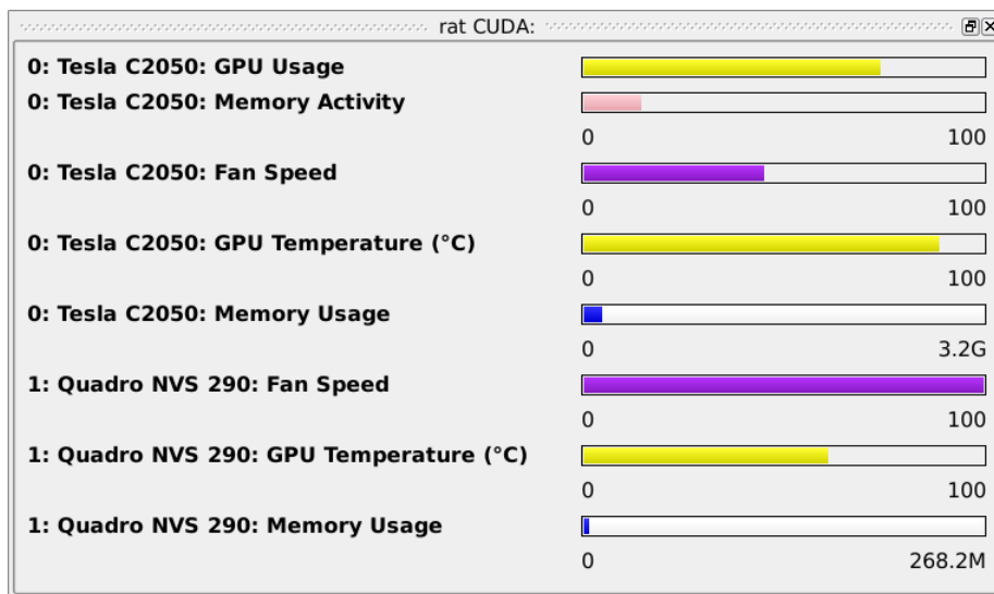
Figure 3-13. CUDA Bar Graph Pane
