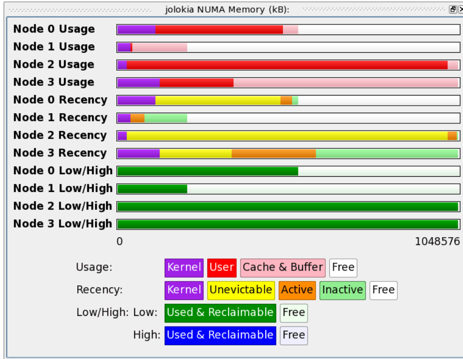
Figure 3-43. NUMA Bar Graph Pane
