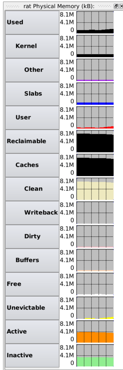
Figure 3-35. Physical Memory Line Graph Pane
