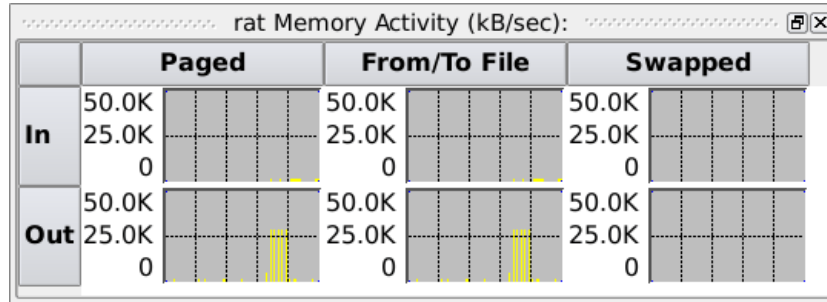
Figure 3-29. Memory Activity Line Graph Pane
