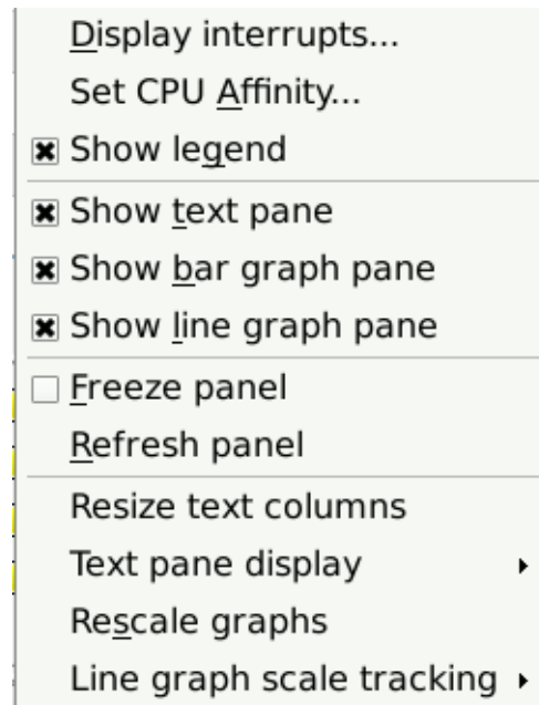
Figure 3-23. Interrupt Activity Context Menu
