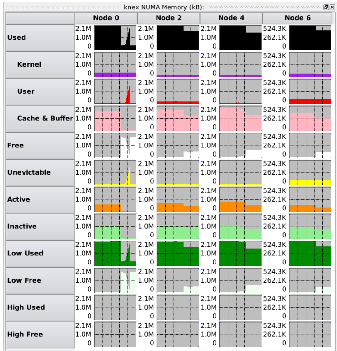
Figure 3-44. NUMA Line Graph Pane
