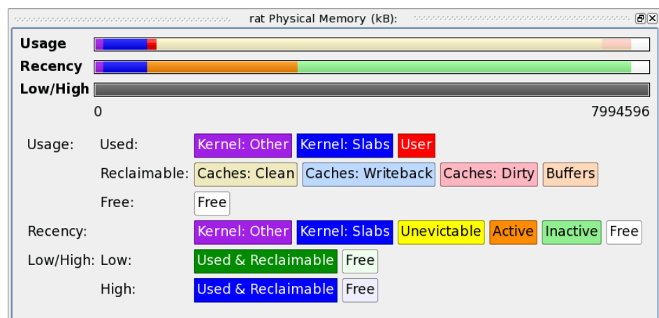
Figure 3-34. Physical Memory Bar Graph Pane
