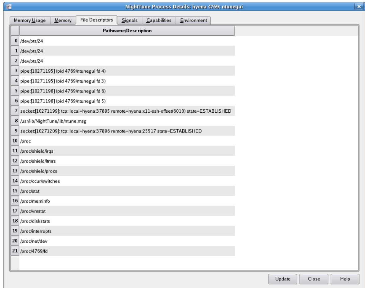
Figure 3-62. Process Details File Descriptors Tab
