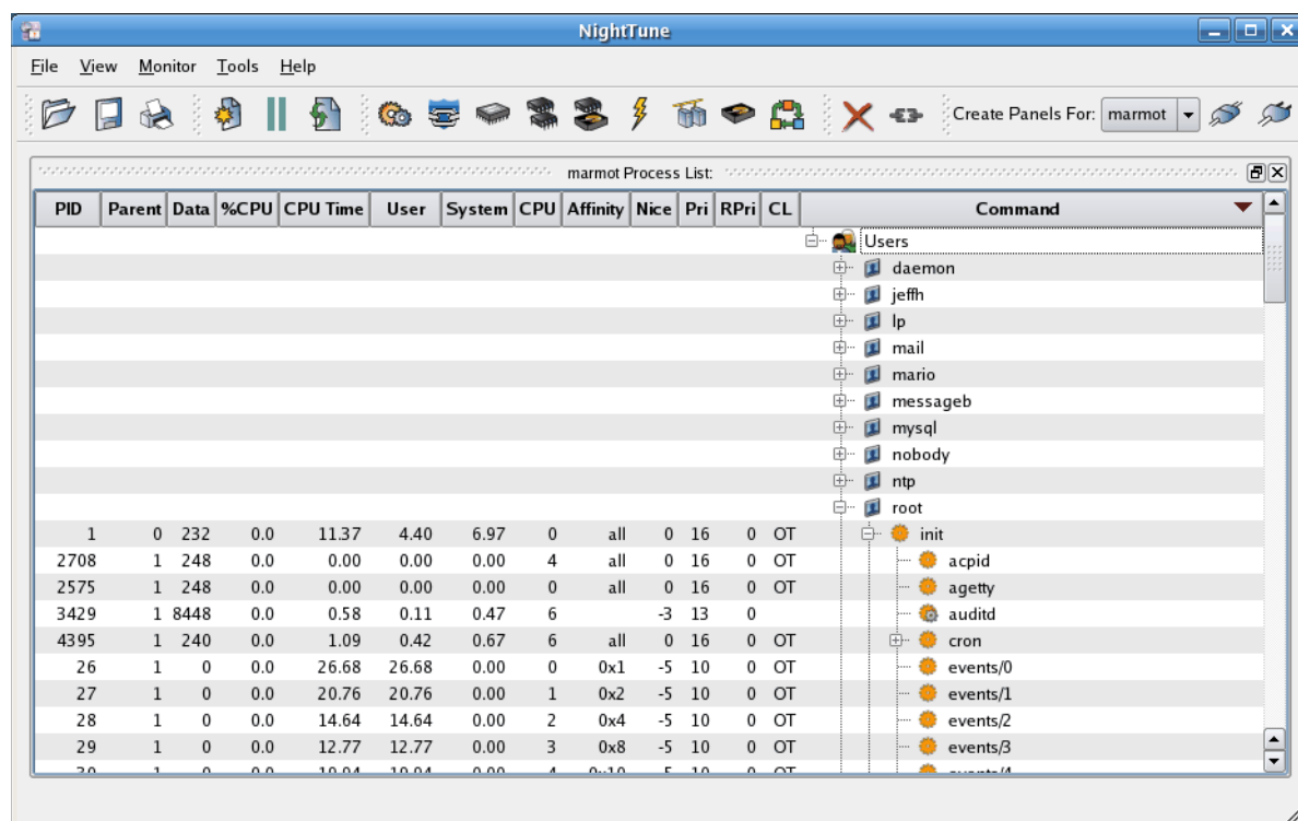
Figure 5-2. Selecting the User Process
