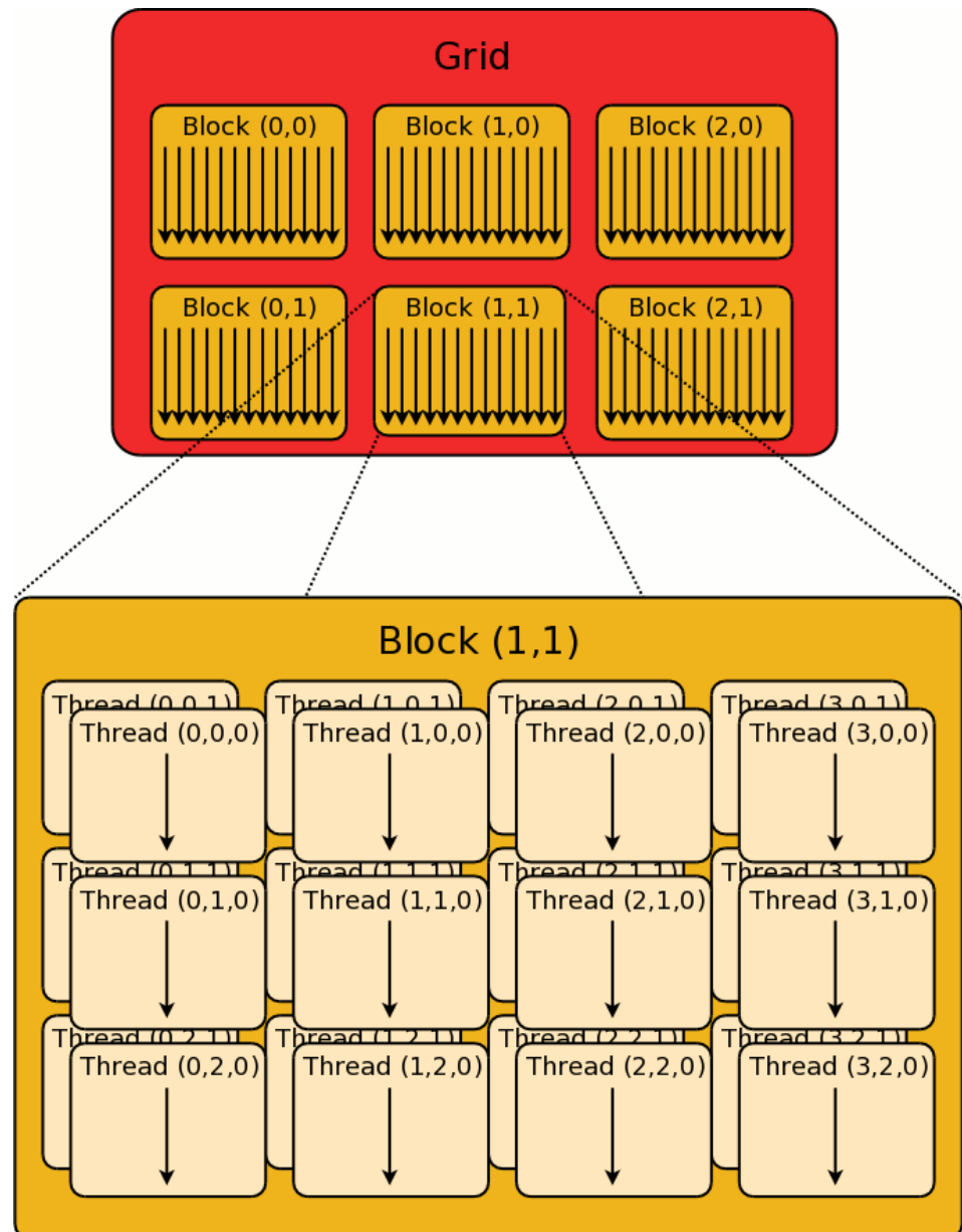
Figure 3-16. Grid, Block, and Thread Hierarchy for \langle\langle 3, 2 \rangle, (4, 3, 2)\rangle
