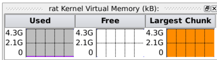
Figure 3-32. Kernel Virtual Memory Line Graph Pane
