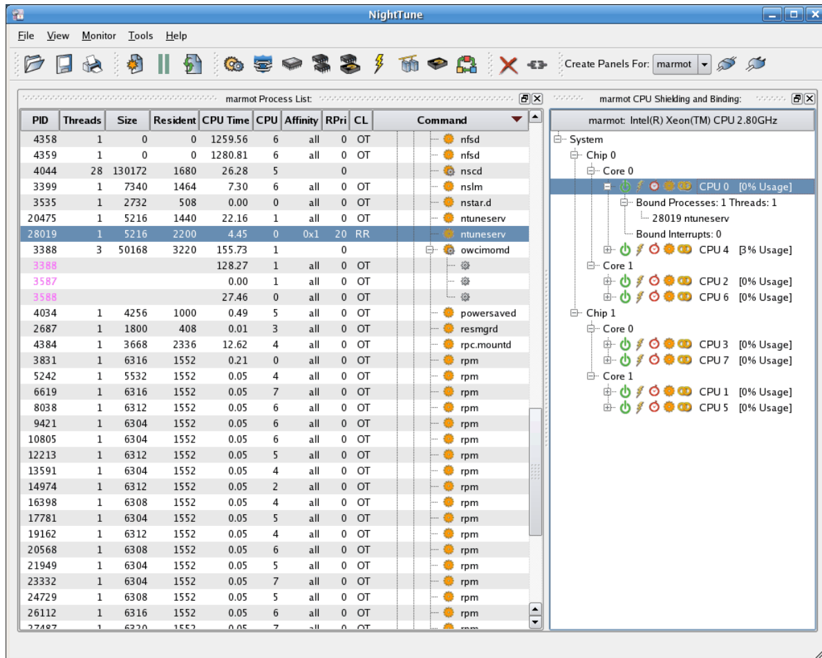
Figure 5-8. Bound Processes
