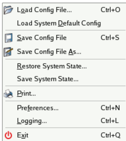
Figure 2-1. File Menu
