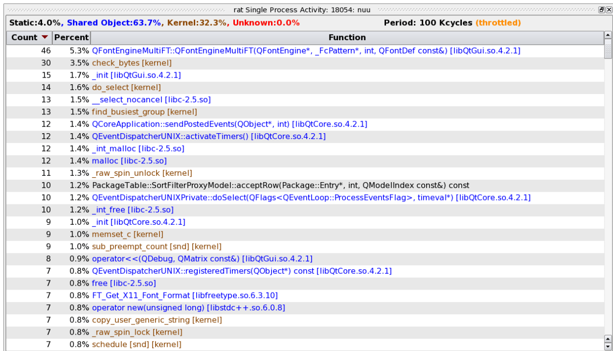
Figure 3-69. Single Process Activity Panel
