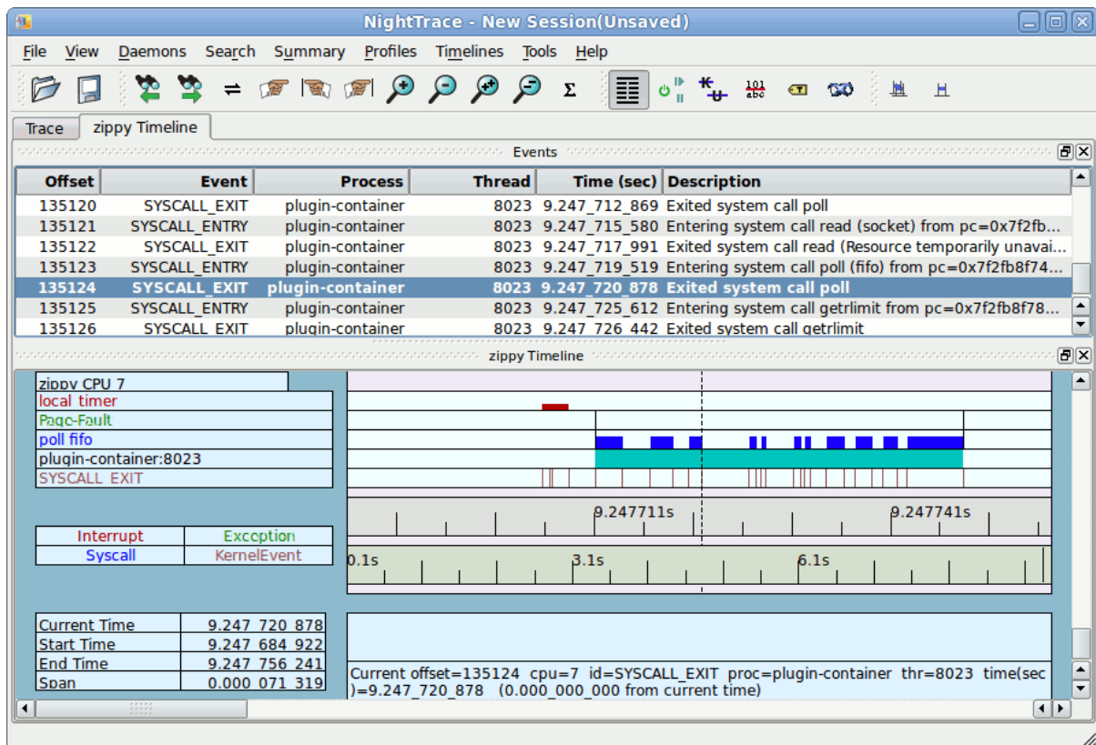
Figure 8-23. Page with Events and Timeline Panels
