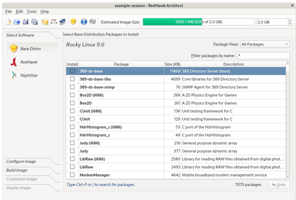
Figure 1-10 Selecting Base Distro Packages, All Packages View
