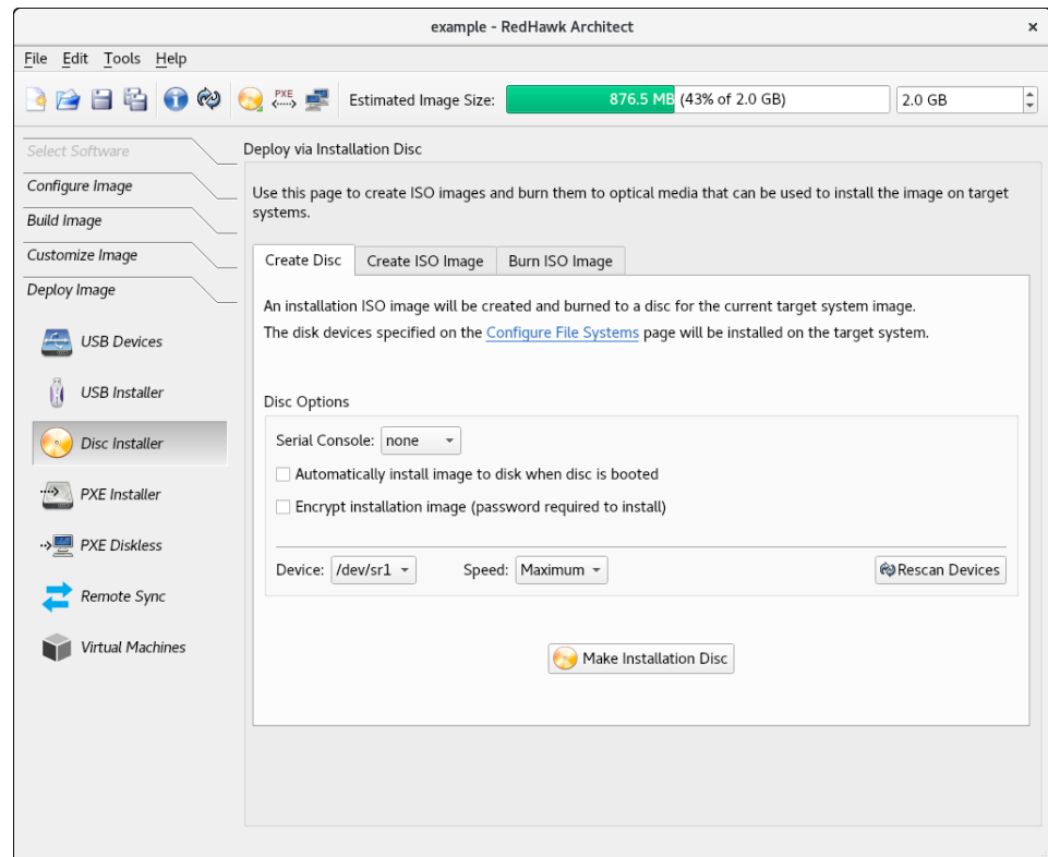
Figure 1-84 Deploy via Installation Disc Page
