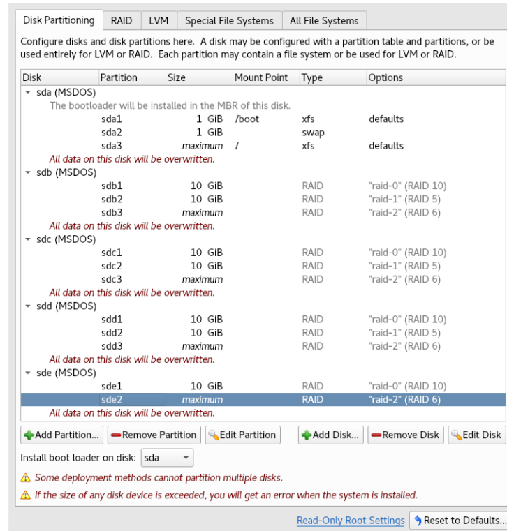
Figure 1-49 Disk partitioning for the three RAIDs configured
