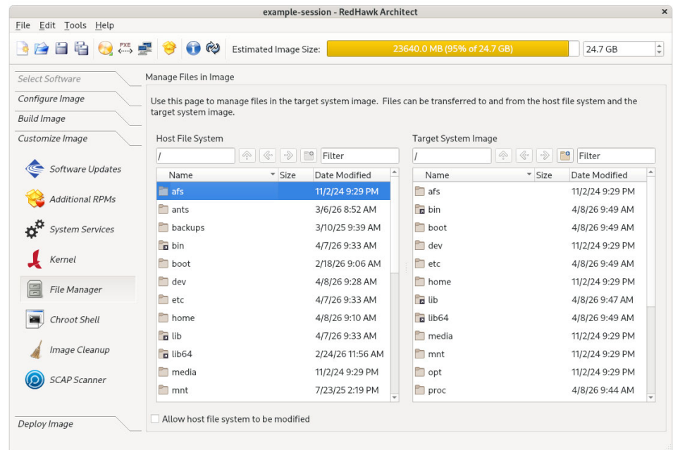
Figure 1-70 Manage Files In Image Page
