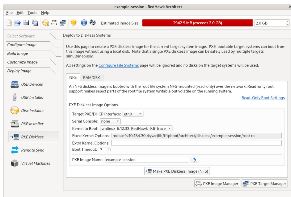
Figure 1-88 Initial PXE RAMDISK Diskless Deployment Page
