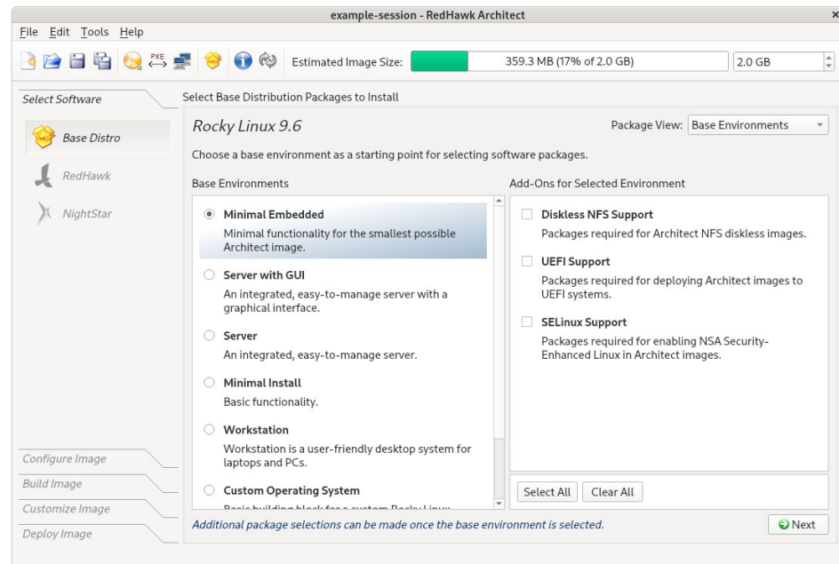
Figure 1-8 Choosing Target Characterization, Base Environments View
