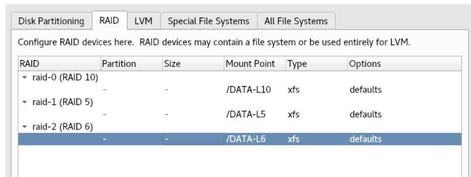
Figure 1-50 RAID tab showing three RAIDs using different RAID levels
