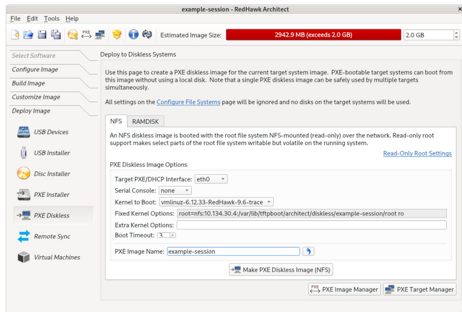
Figure 1-87 Initial PXE NFS Diskless Deployment Page
