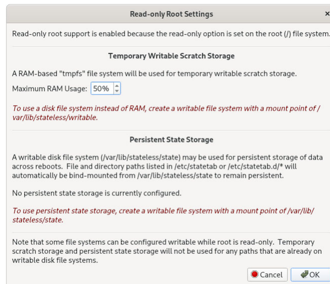
Figure 1-51 Modifiable Maximum RAM Usage setting
