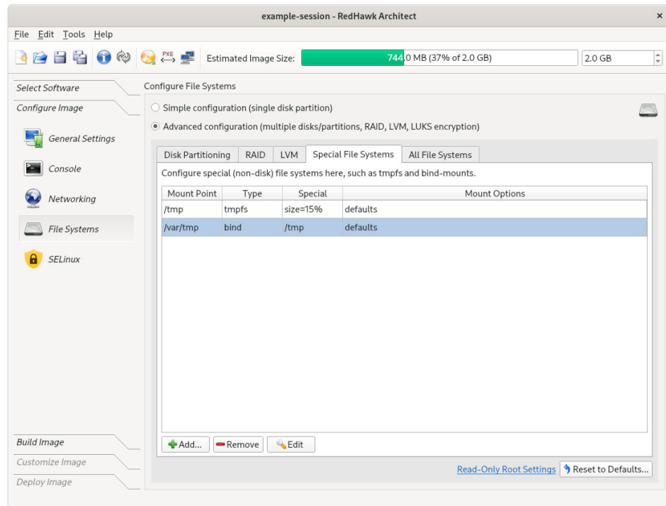
Figure 1-53 Example Special File Systems page entries
