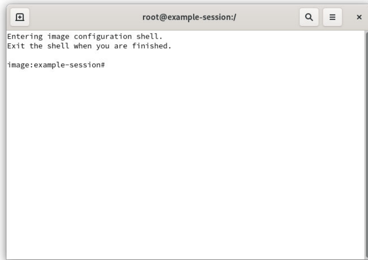
Figure 1-72 chroot Shell
