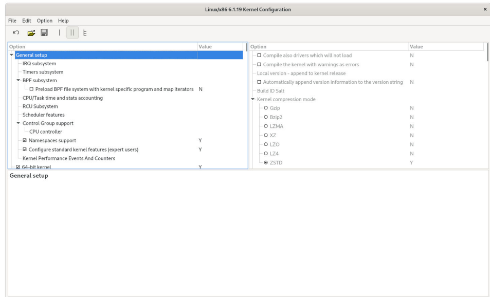
Figure 1-66 Linux Kernel Configuration Dialog
