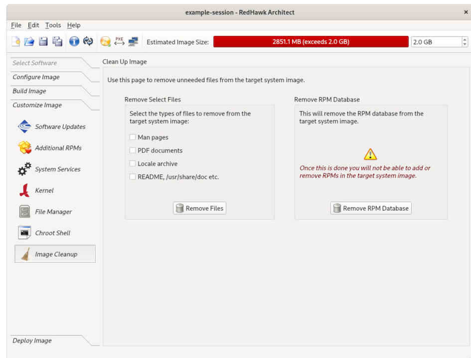
Figure 1-73 Clean Up Image Page
