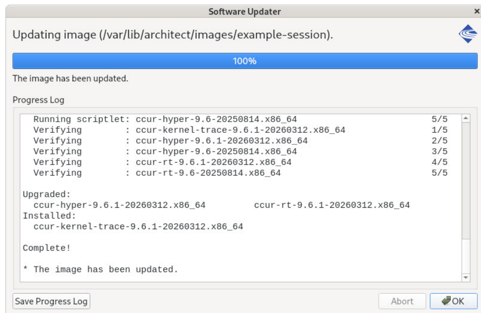
Figure 1-61 Software Updater Dialog
