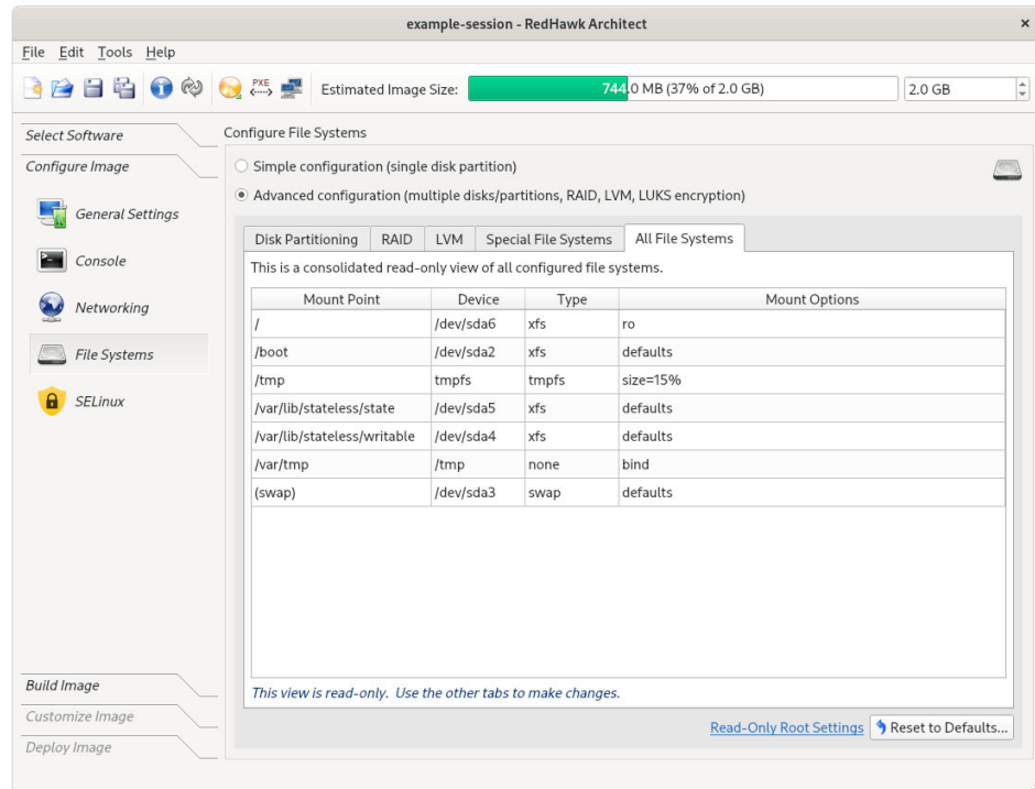
Figure 1-54 Example All File Systems list
