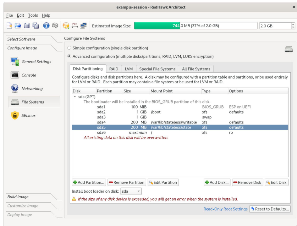
Figure 1-52 Example root read-only partitioning scheme
