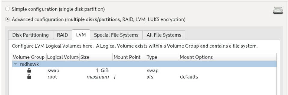
Figure 1-48 LVM configuration with LUKS encryption
