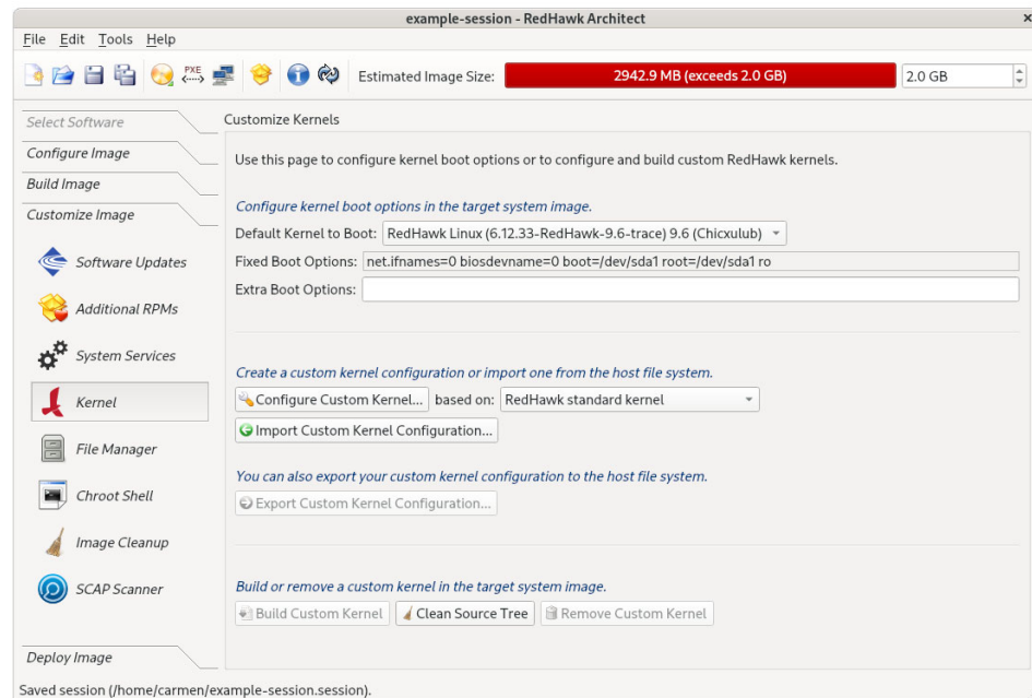
Figure 1-64 Customize Kernels Page
