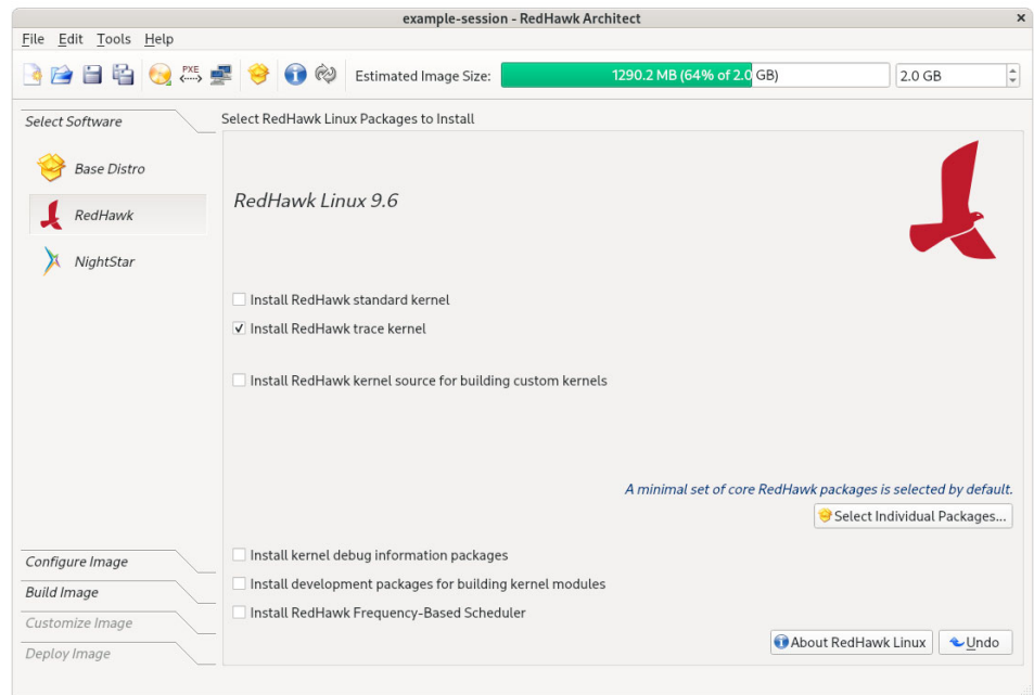
Figure 1-12 Selecting RedHawk Options
