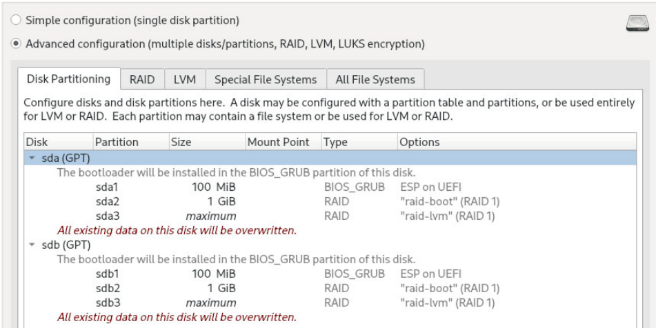
Figure 1-47 Disk devices for RAID ‘RAID 1’created
