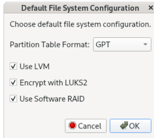
Figure 1-46 Default File System Configuration
