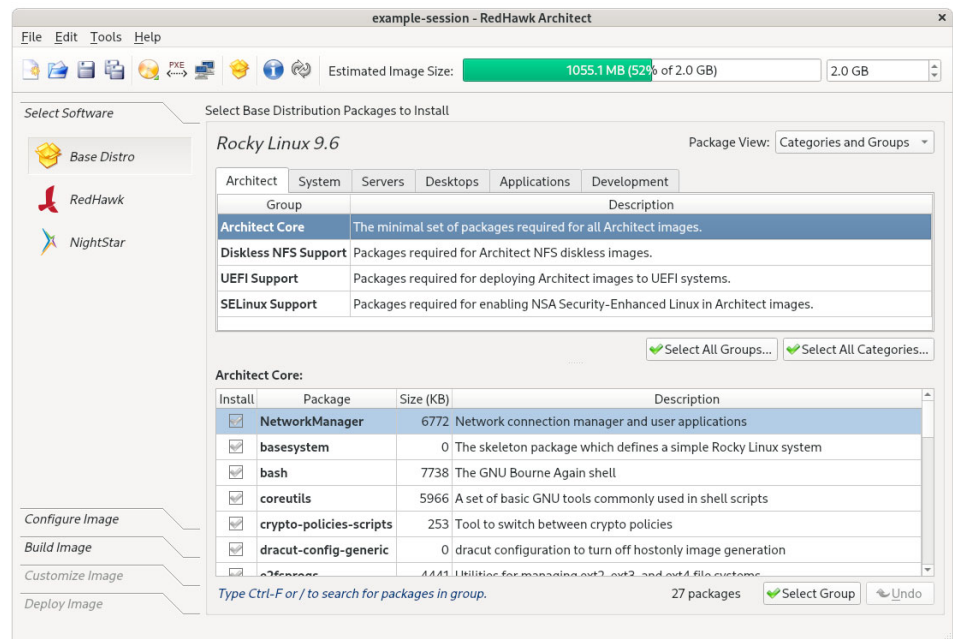
Figure 1-9 Selecting Base Distro Packages, Categories and Groups View
