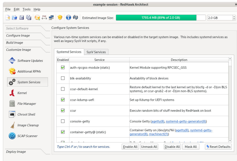
Figure 1-63 System Services Page
