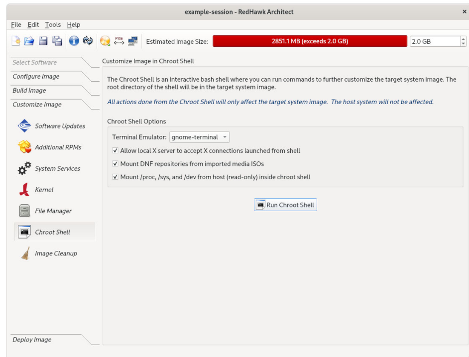
Figure 1-71 Chroot Shell Page
