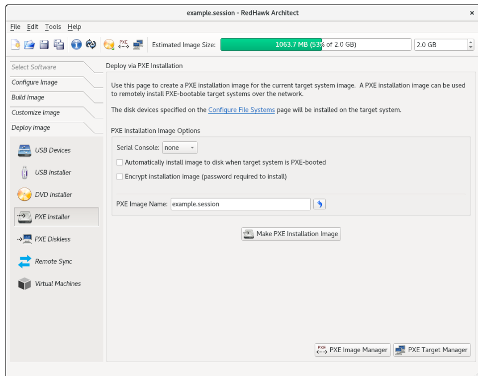
Figure 1-85 Deploy via PXE Installation Page
