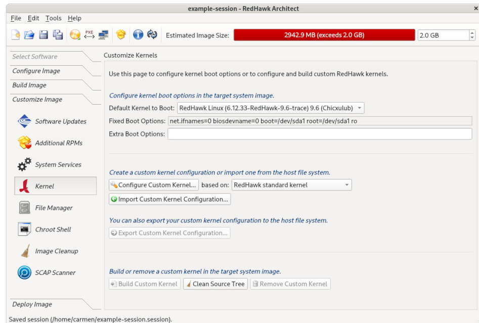
Figure 1-65 Customize Kernels Page
