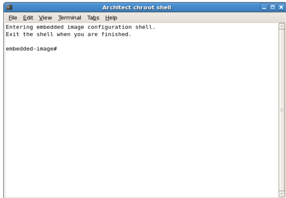
Figure 1-32 chroot Shell
