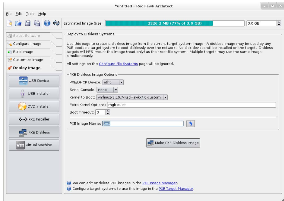
Figure 1-56 PXE Diskless Deployment Page
