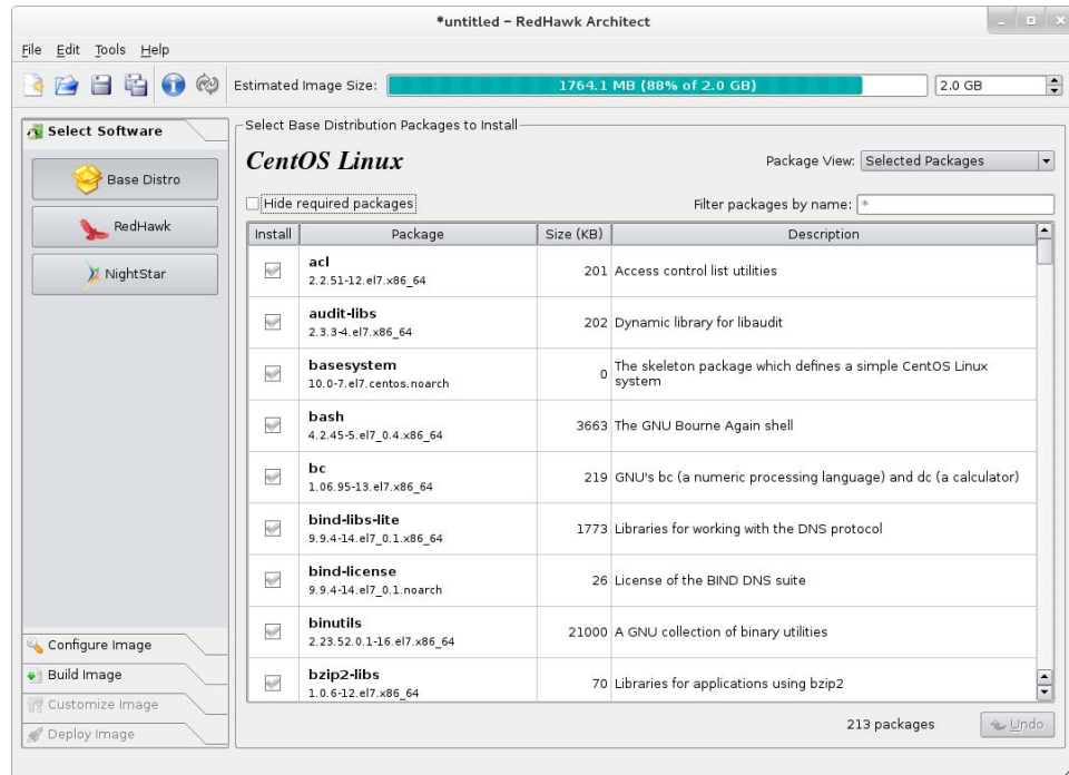
Figure 1-7 Selecting Base Distro Packages, Selected Packages View
