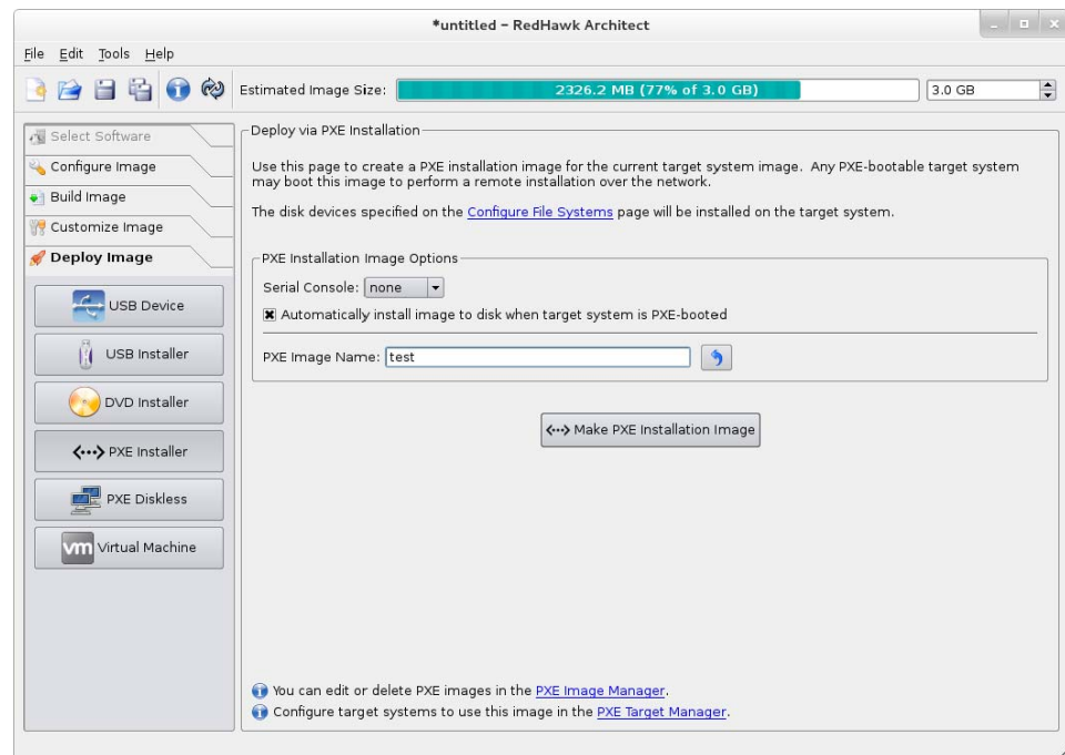
Figure 1-52 Deploy via PXE Installation Page
