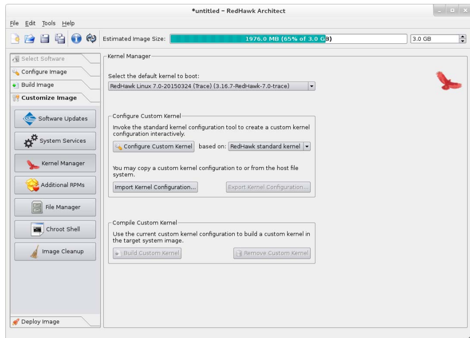
Figure 1-32 Kernel Manager Page
