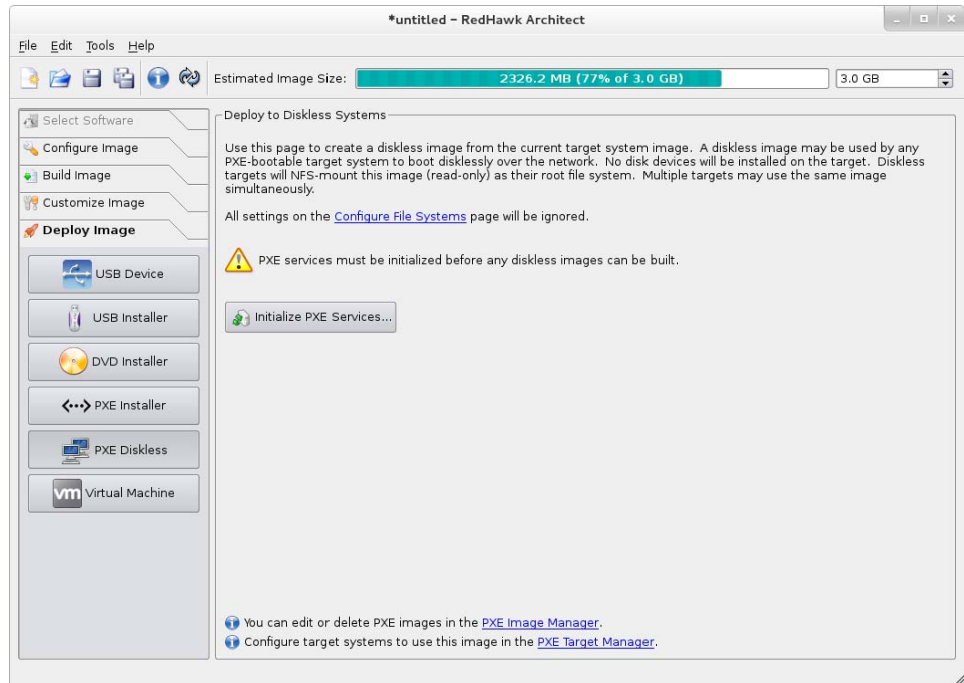
Figure 1-55 Initial PXE Diskless Deployment Page
