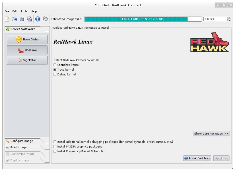
Figure 1-8 Selecting RedHawk Options
