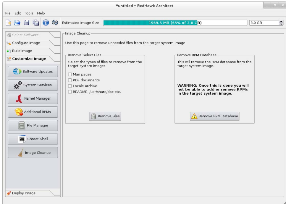
Figure 1-43 Image Cleanup Page
