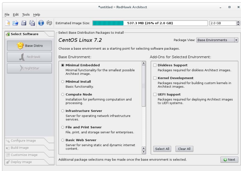
Figure 1-5 Choosing Target Characterization, Base Environments View
