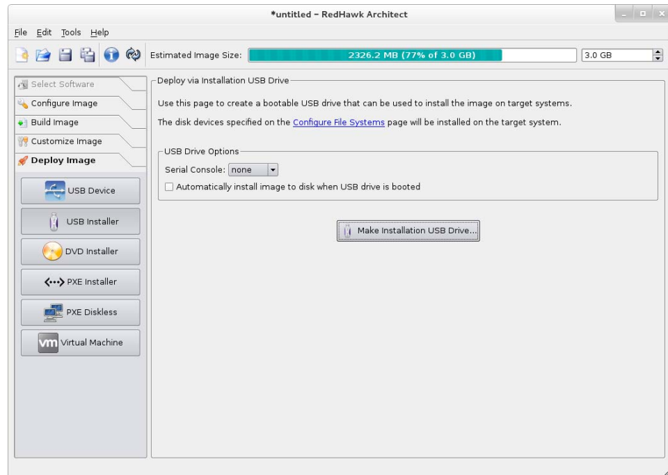
Figure 1-51 Deploy via Installation USB Drive Page
