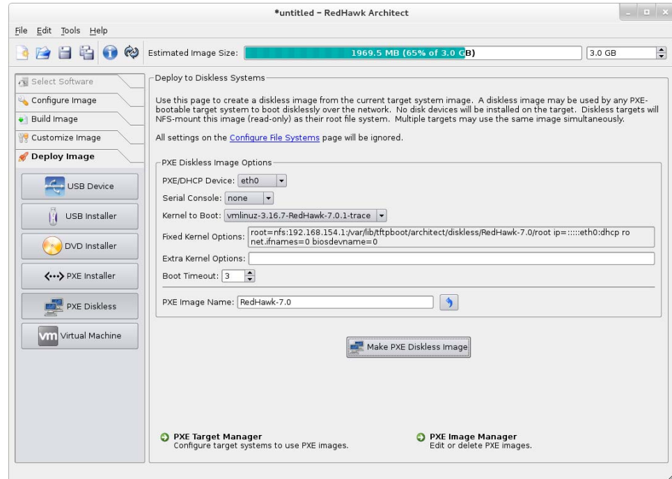
Figure 1-57 PXE Diskless Deployment Page
