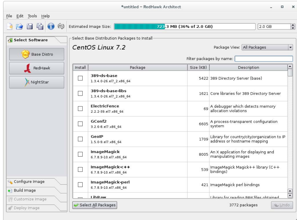
Figure 1-7 Selecting Base Distro Packages, All Packages View
