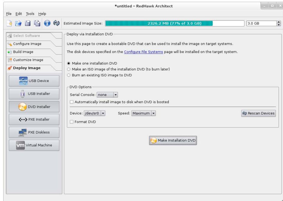
Figure 1-52 Deploy via Installation DVD Page
