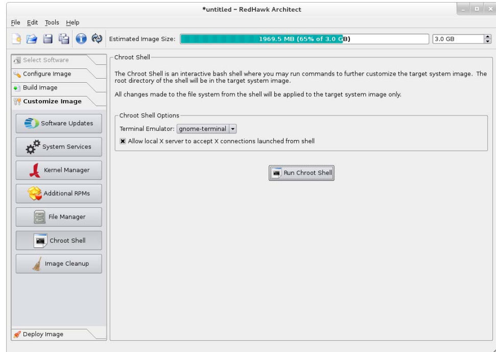
Figure 1-41 Chroot Shell Page
