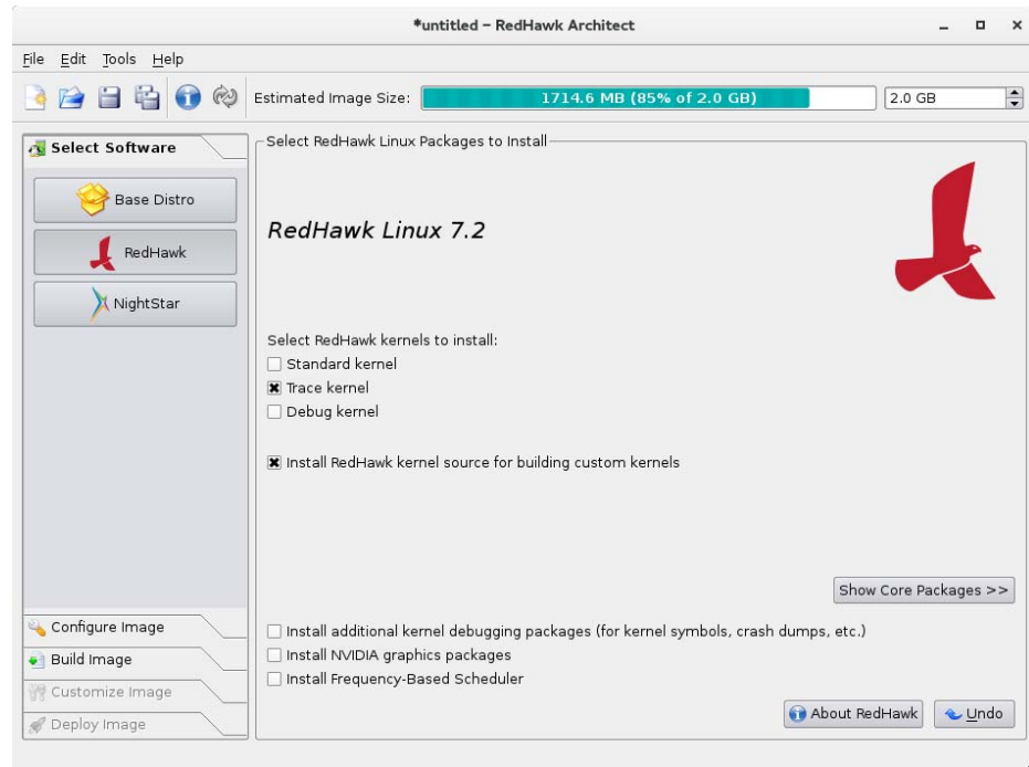
Figure 1-9 Selecting RedHawk Options
