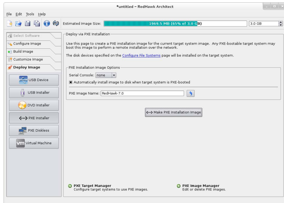
Figure 1-53 Deploy via PXE Installation Page
