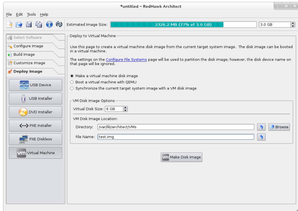
Figure 1-60 Deploy to Virtual Machine Page
