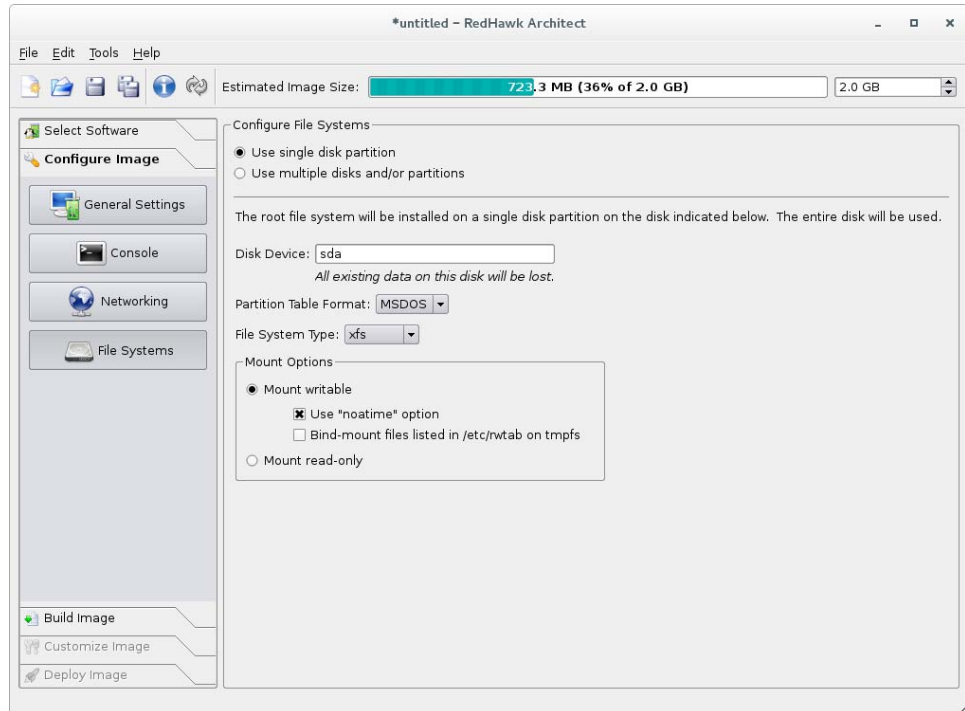
Figure 1-18 File System Configuration Page
