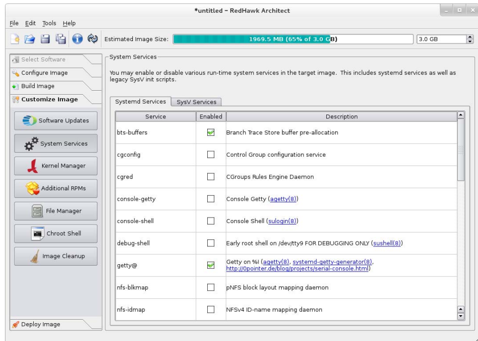
Figure 1-32 System Services Page
