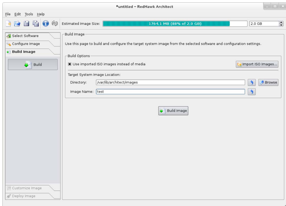
Figure 1-20 Build Image Page
