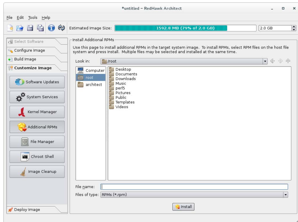
Figure 1-39 Install Additional RPMs Page
