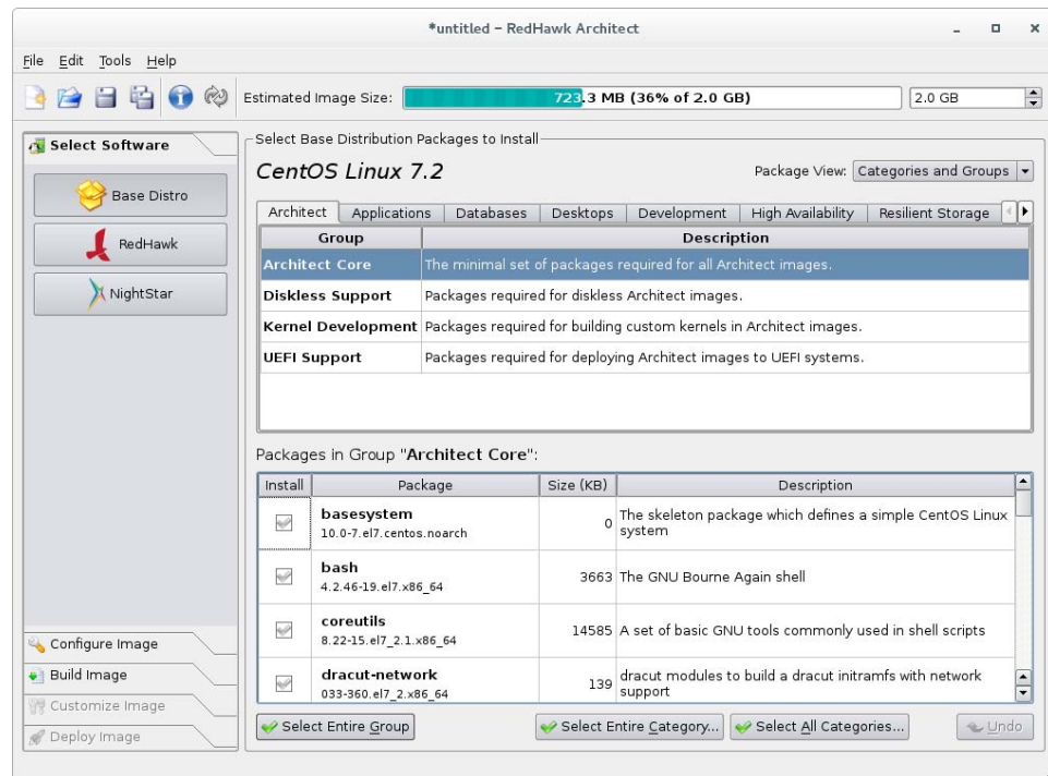
Figure 1-6 Selecting Base Distro Packages, Categories and Groups View
