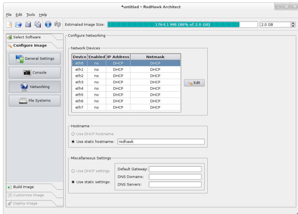
Figure 1-15 Network Configuration Page
