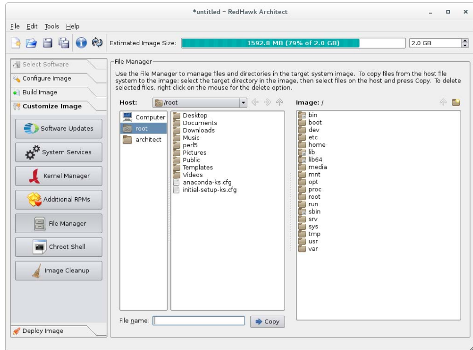
Figure 1-40 File Manager Page
