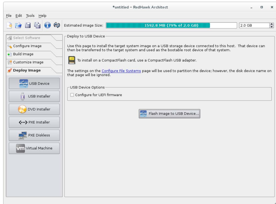
Figure 1-44 Deploy to USB Device Page
