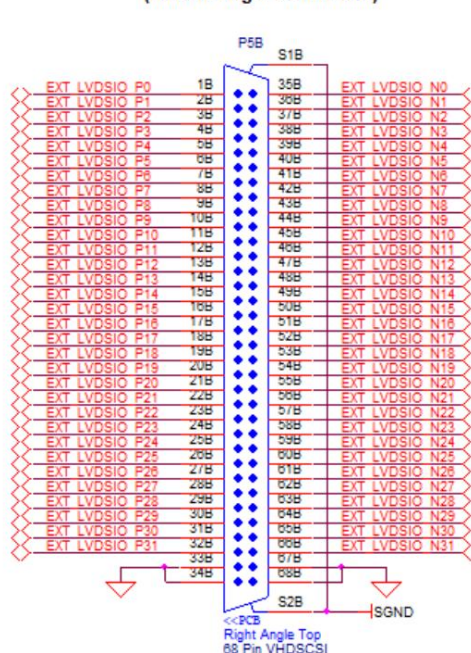
LVDS Input/Output Connector (Bottom Right Connector)
