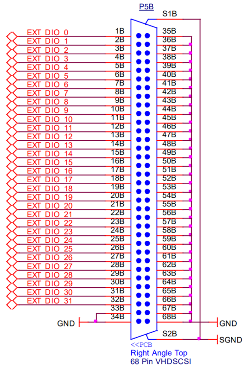
Daughter Card #2 Input/Output Connector (Top Right Connector)
