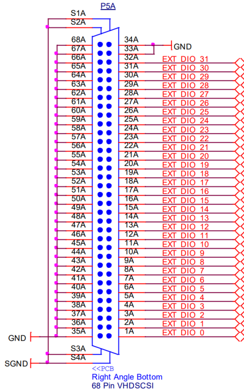
Daughter Card #1 Input/Output Connector (Top Left Connector)
