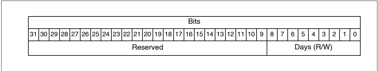
Figure A-60 RCIM IV IRIG Output Years Register
