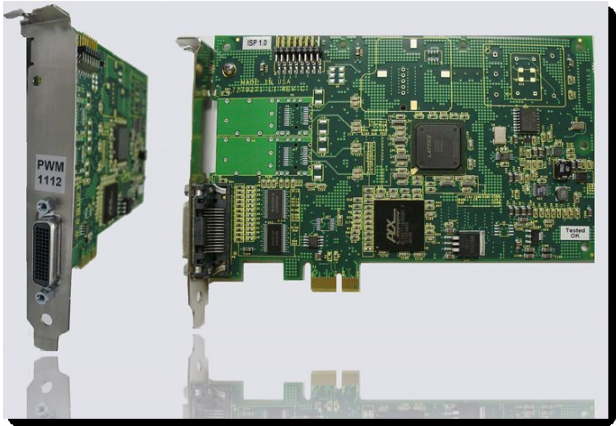
Figure 6. CP-PWM-1112 Card
