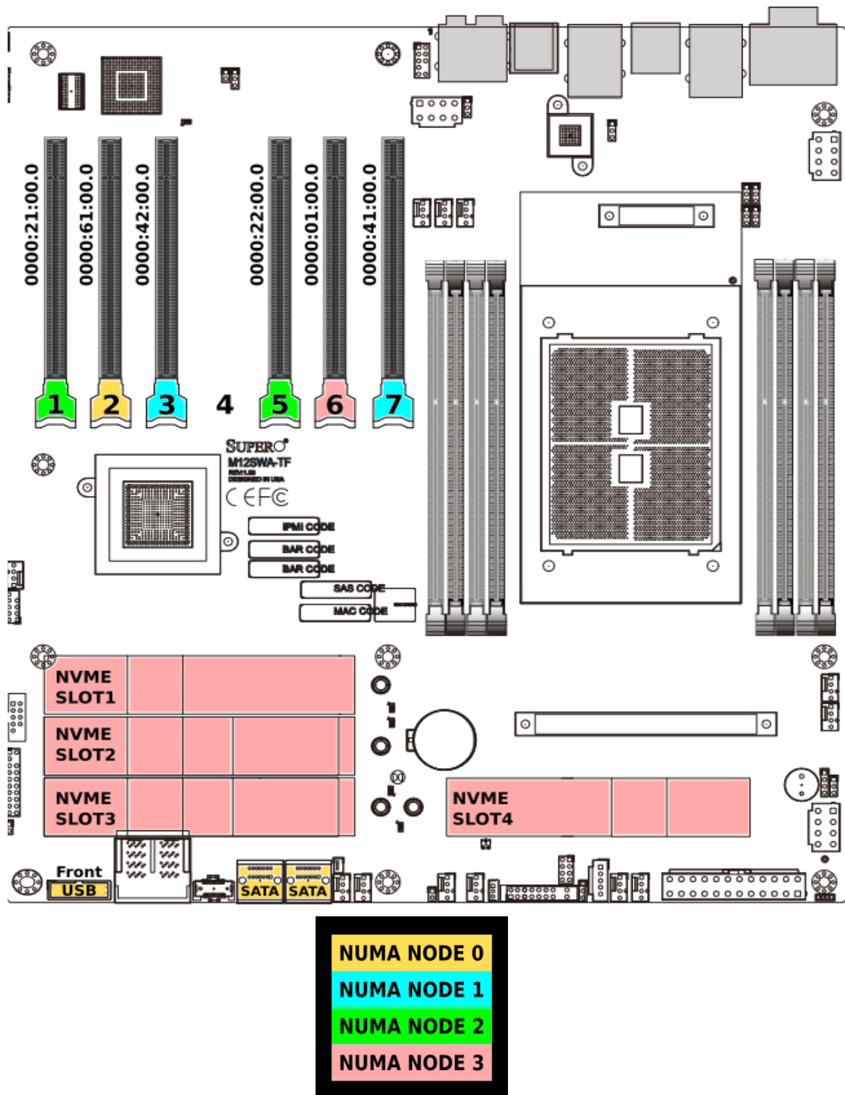
Figure A-1 NUMA node mapping of devices in the Supermicro M12SWA-TF
