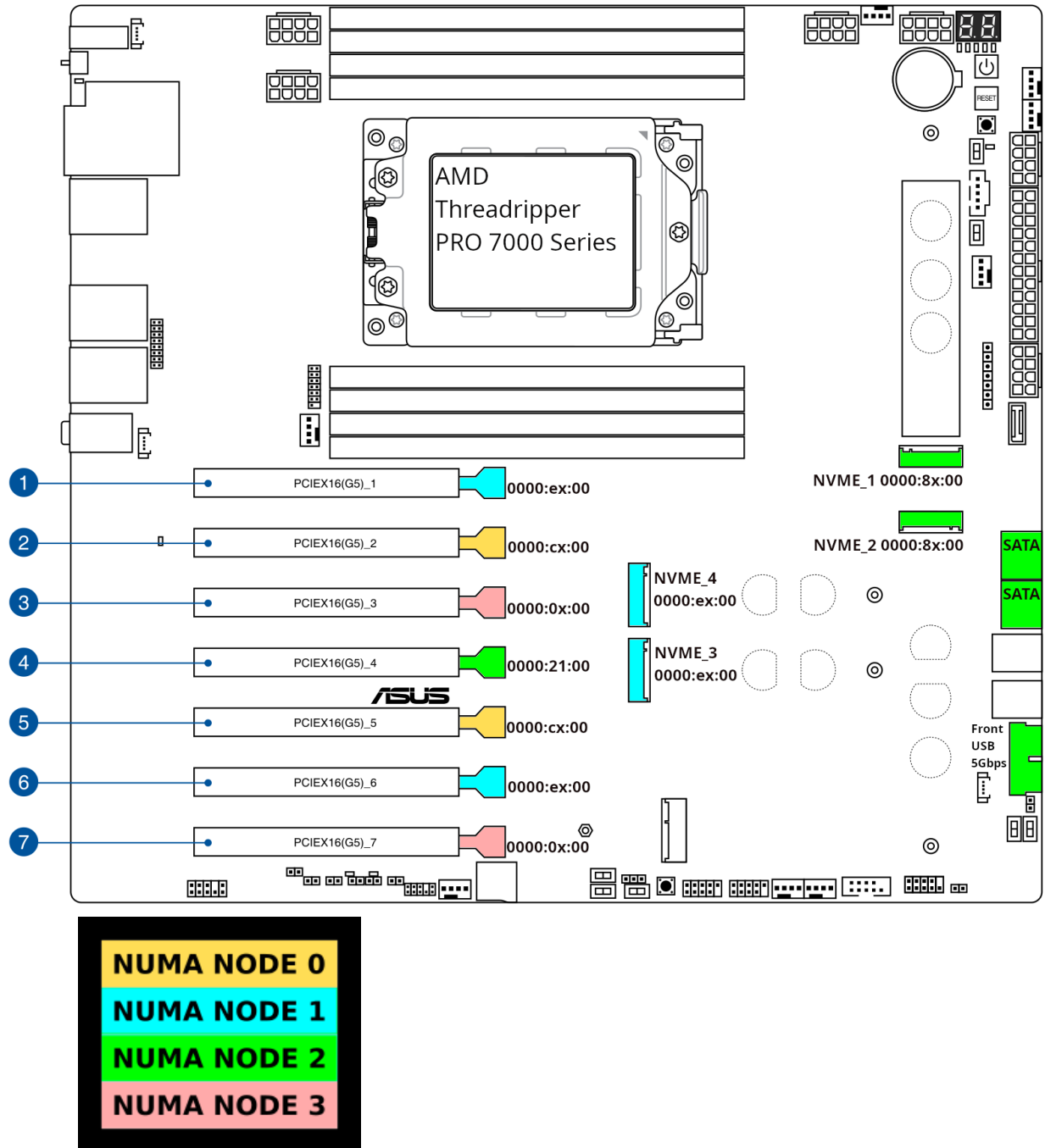
Figure A-3 NUMA Node Mapping of Devices in the ASUS Pro WS WRX90E-SAGE SE
