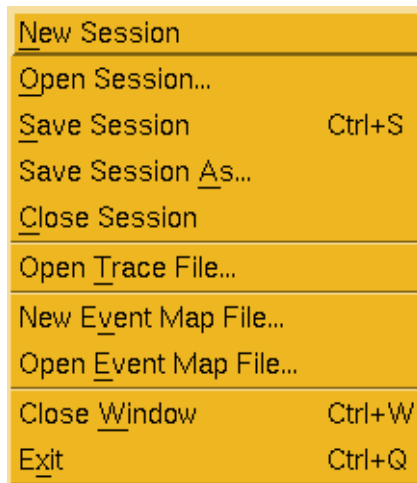
Figure 3-2. NightTrace menu
