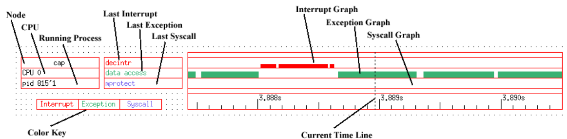
Figure 13-4. Per-CPU Information
