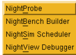
Figure 3-17. Tools menu
