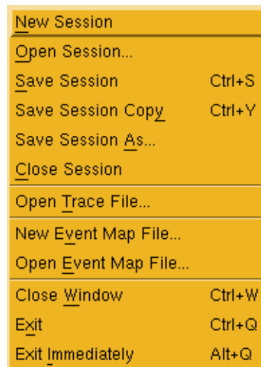
Figure 3-2. NightTrace menu
