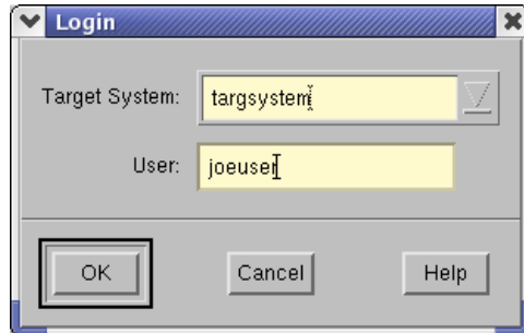
Figure 3-6. Login dialog
