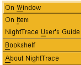
Figure 3-18. Help menu
